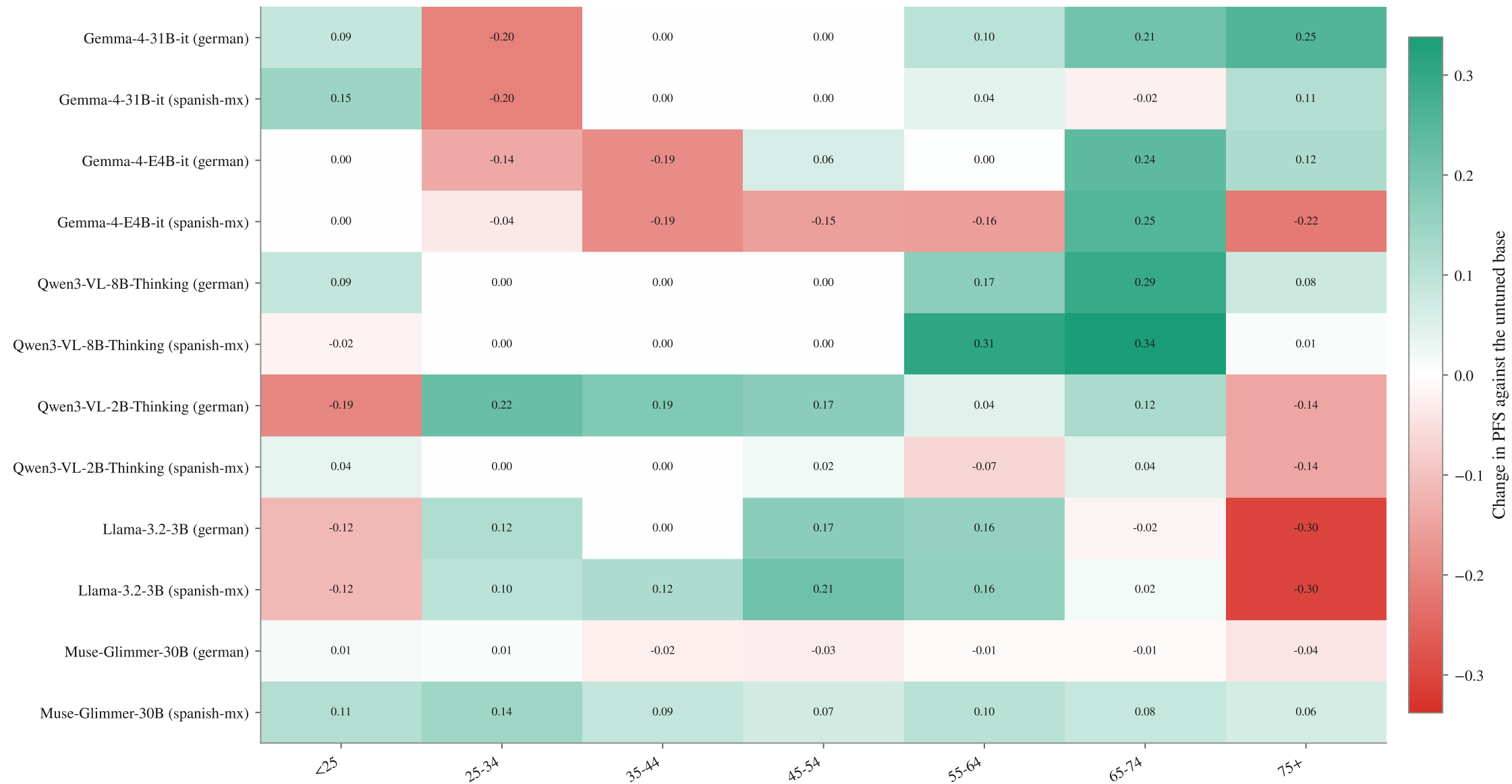
Finetuning change in fidelity — Age band, religious, NTP
