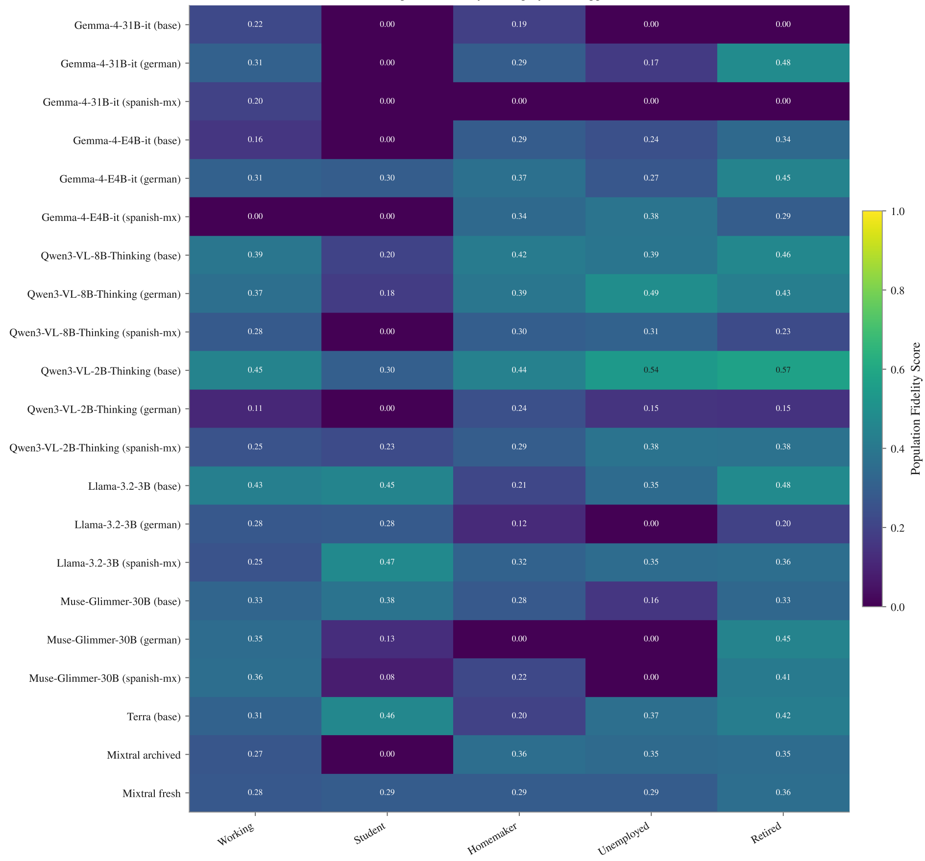
Population fidelity — Employment, happiness, FA
