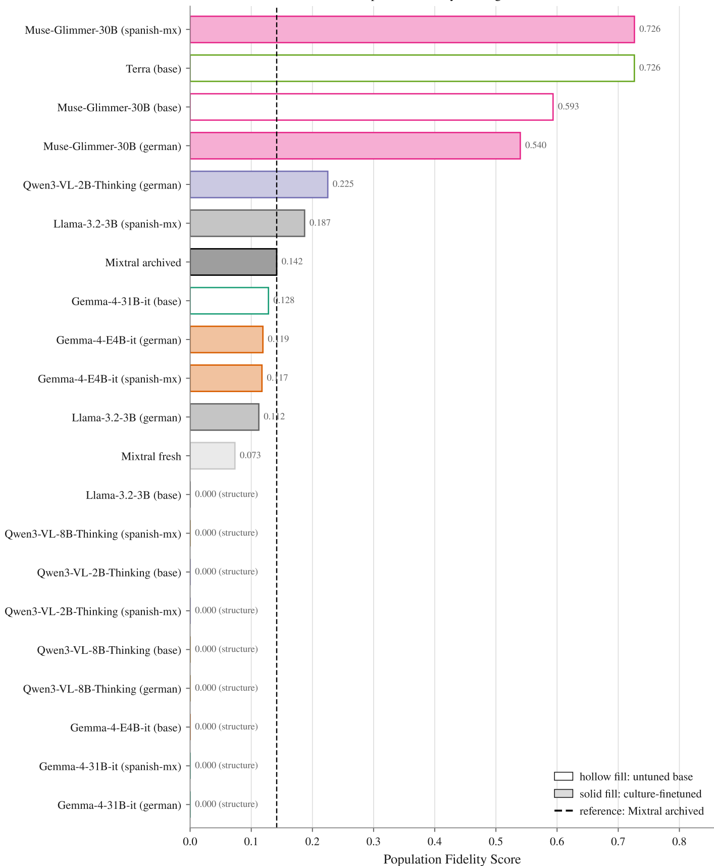
Population fidelity — religious, FA
