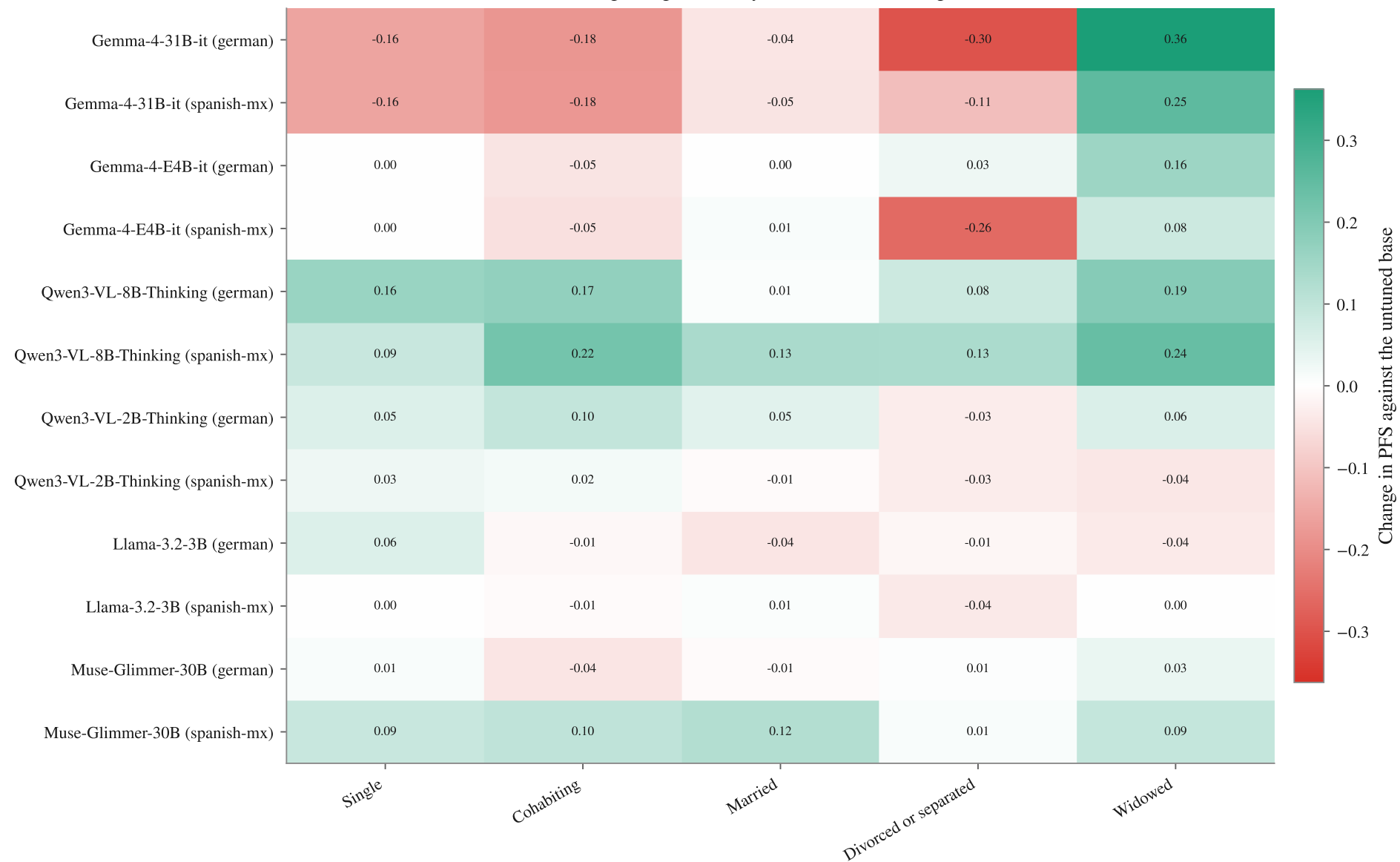
Finetuning change in fidelity — Marital status, religious, NTP
