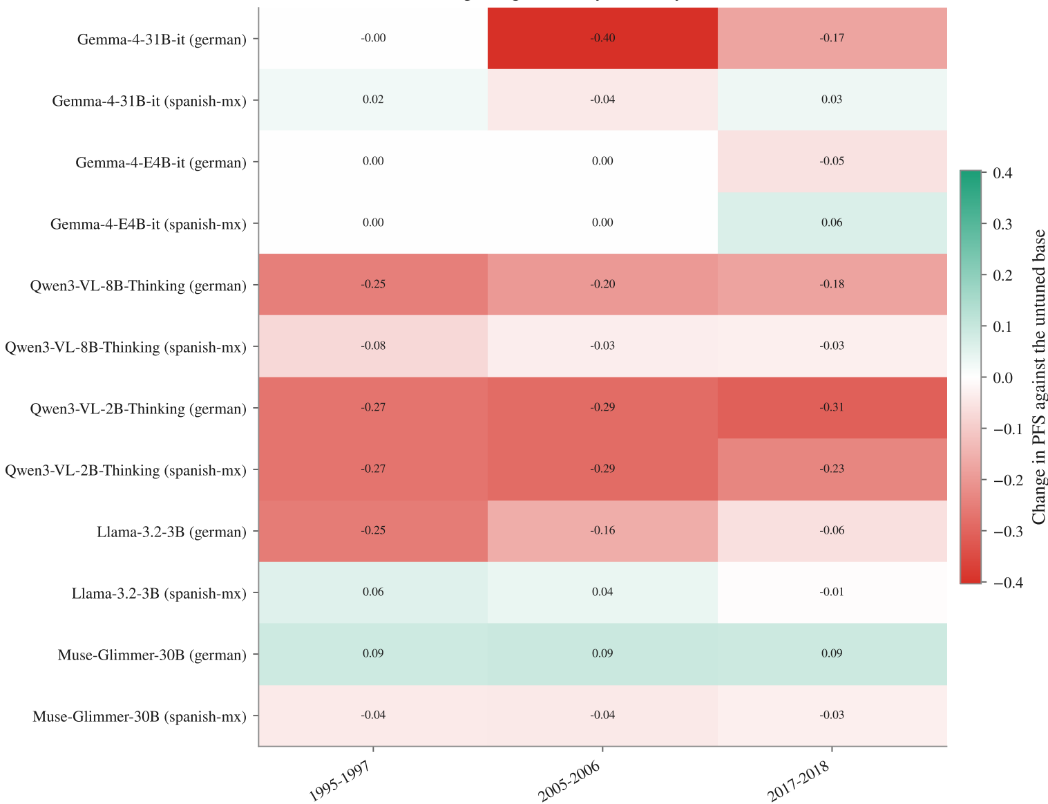
Finetuning change in fidelity — Survey wave, trust, NTP
