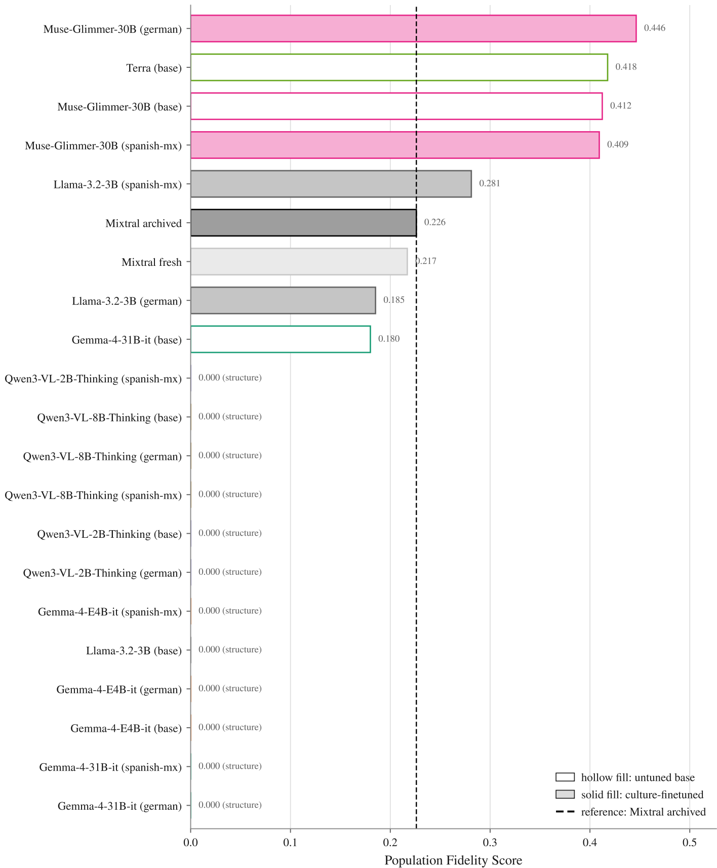
Population fidelity — every topic, FA
