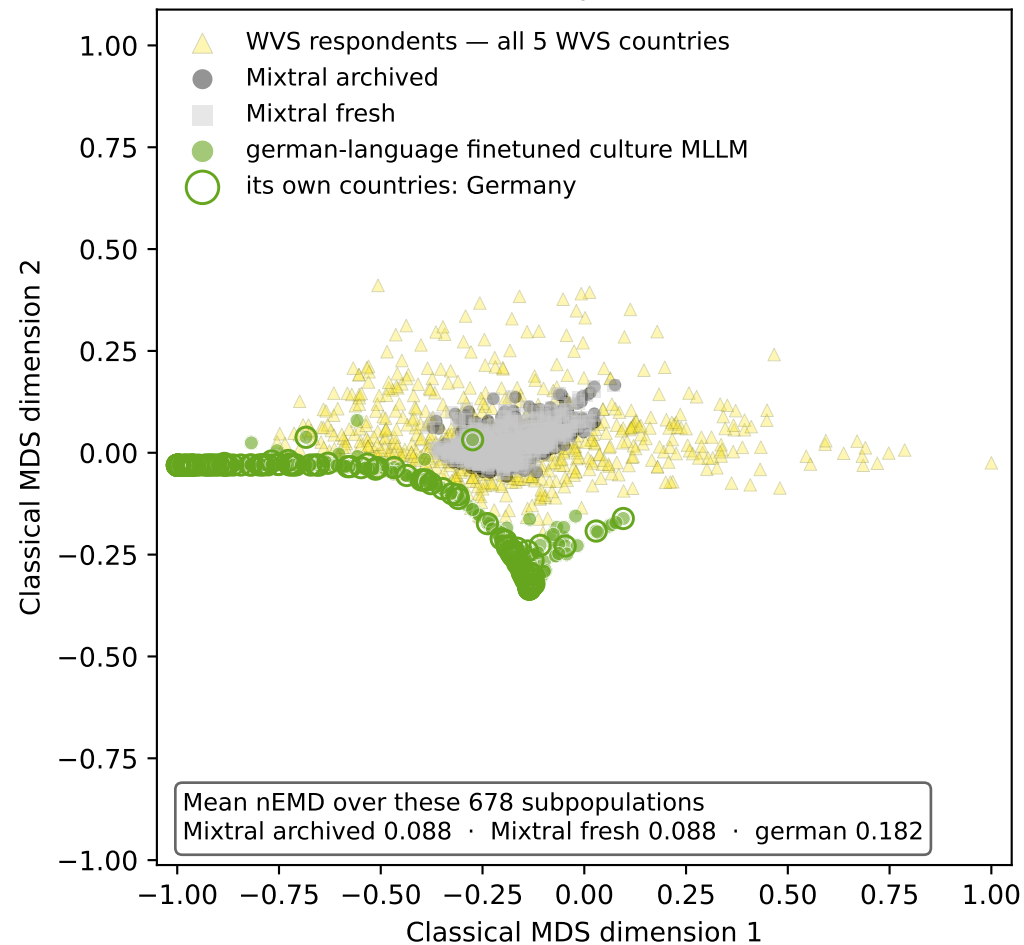
Next-token probabilities
