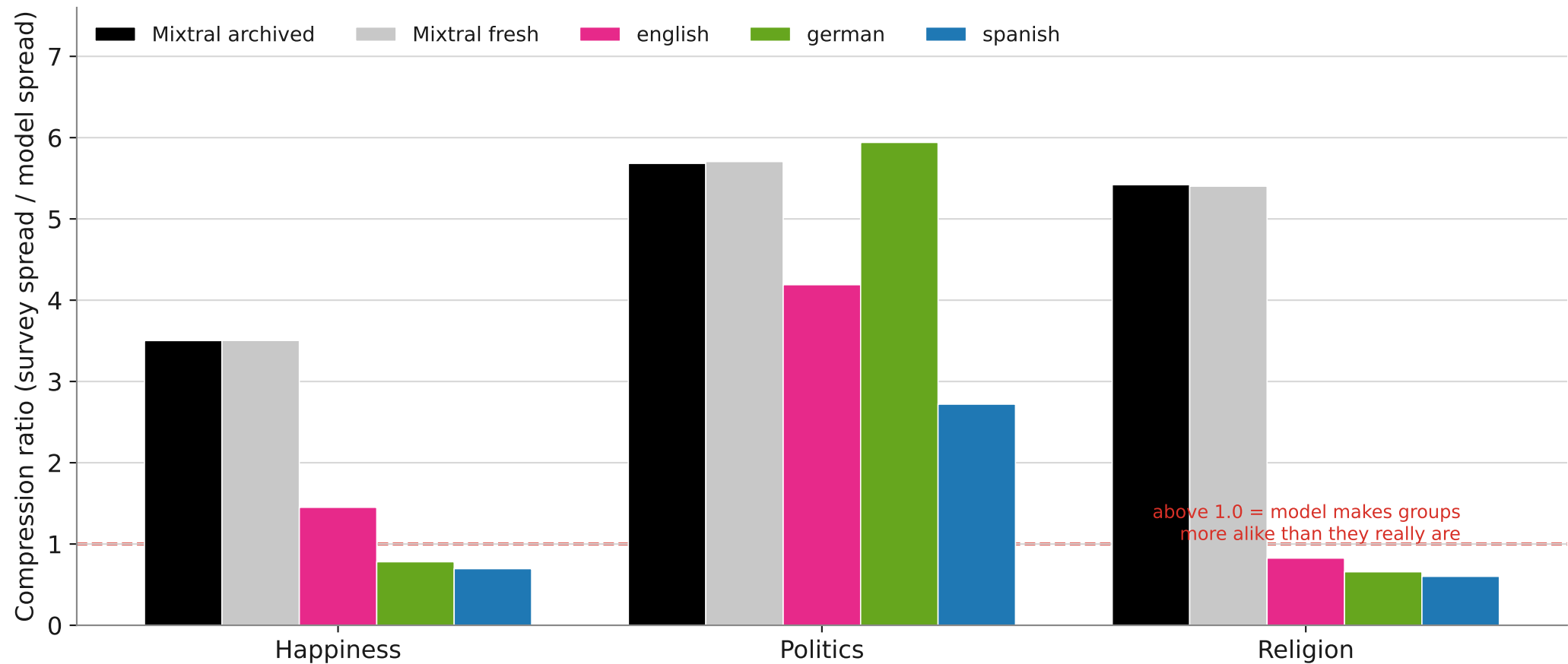
How much the model flattens the differences between groups
