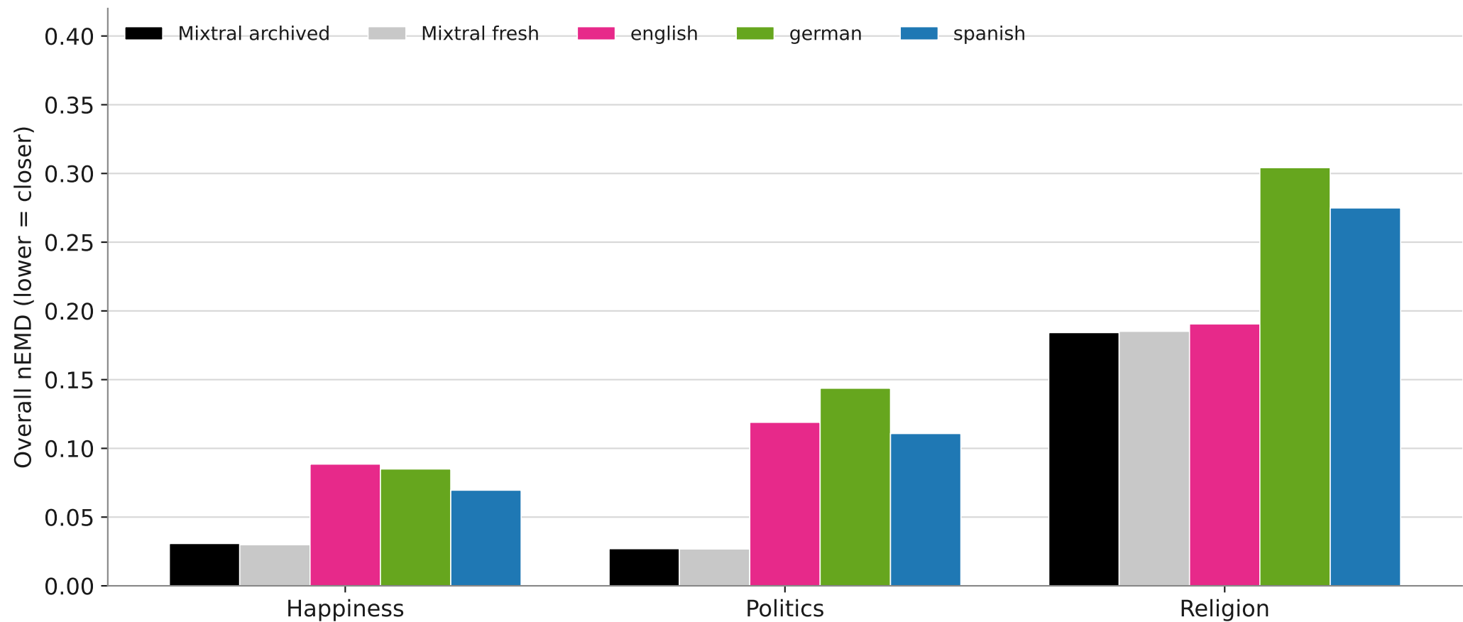
Distance from the survey's answer distribution
