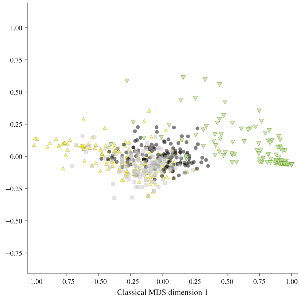
FA · 144 subpopulations · mean nEMD Mixtral archived 0.092, Mixtral fresh 0.074, german 0.268
