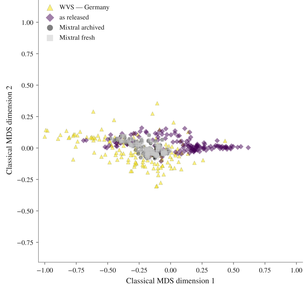
FA · 144 subpopulations · mean nEMD base 0.116, Mixtral archived 0.092, Mixtral fresh 0.074
