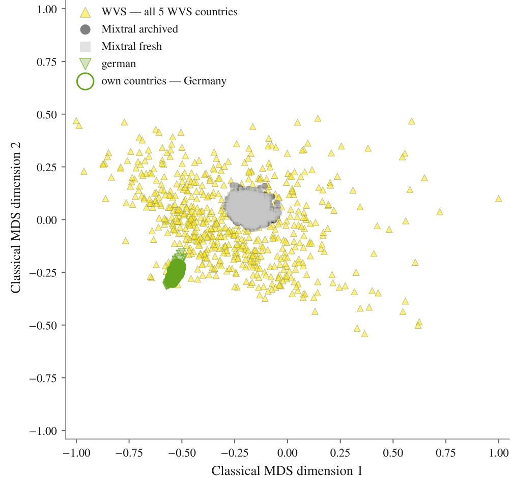
NTP · 639 subpopulations · mean nEMD Mixtral archived 0.090, Mixtral fresh 0.090, german 0.121
