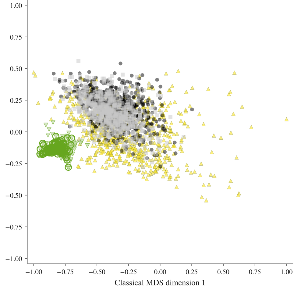
FA · 639 subpopulations · mean nEMD Mixtral archived 0.108, Mixtral fresh 0.107, german 0.165
