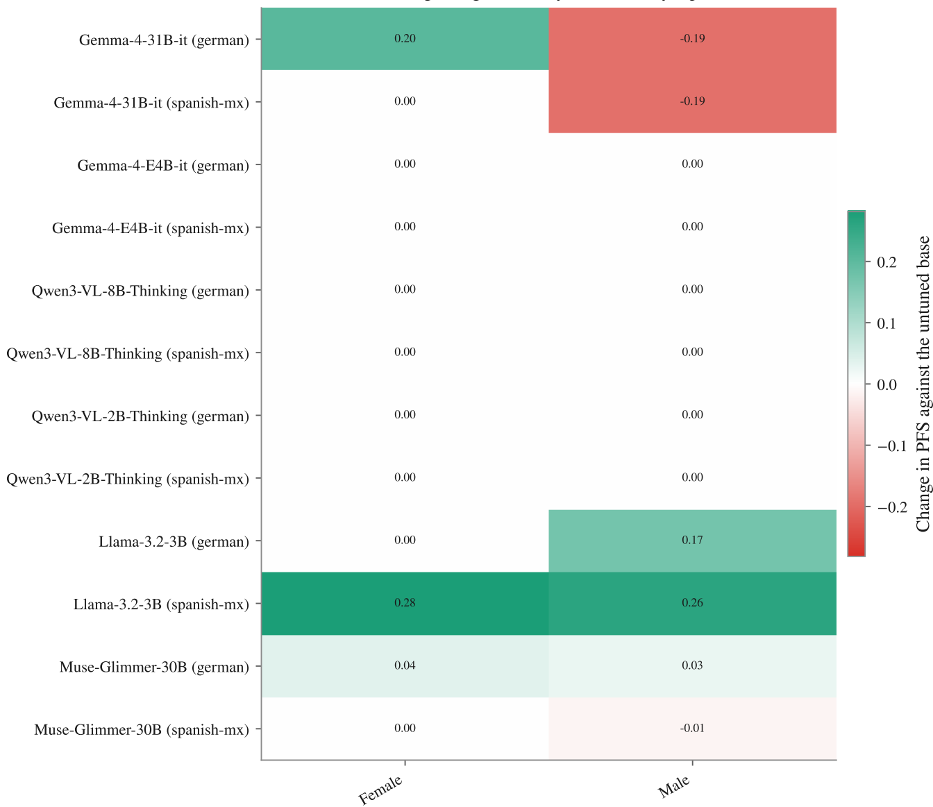
Finetuning change in fidelity — Sex, every topic, FA
