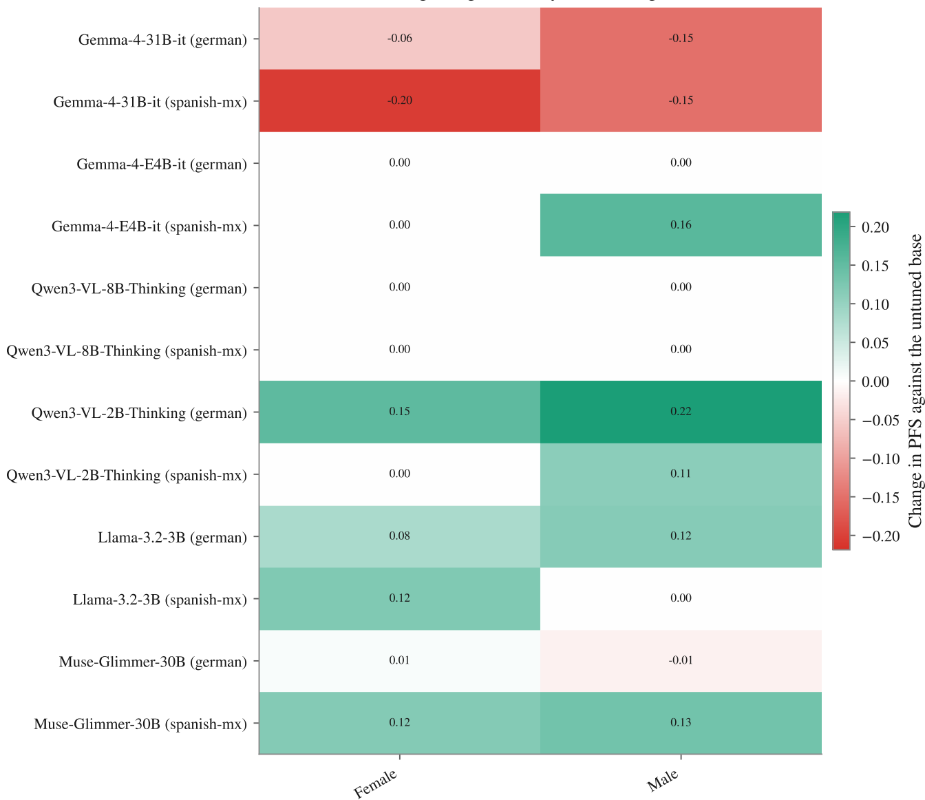
Finetuning change in fidelity — Sex, religious, NTP
