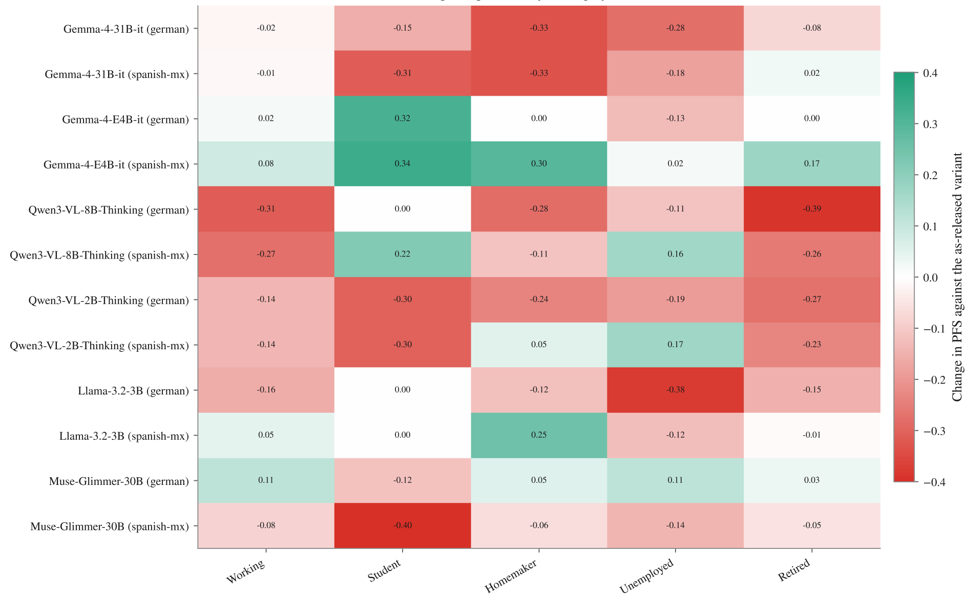
Finetuning change in fidelity — Employment, trust, FA
