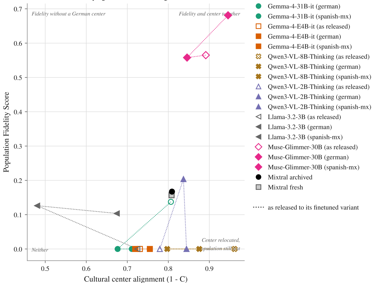
Fidelity against center — religious, NTP
