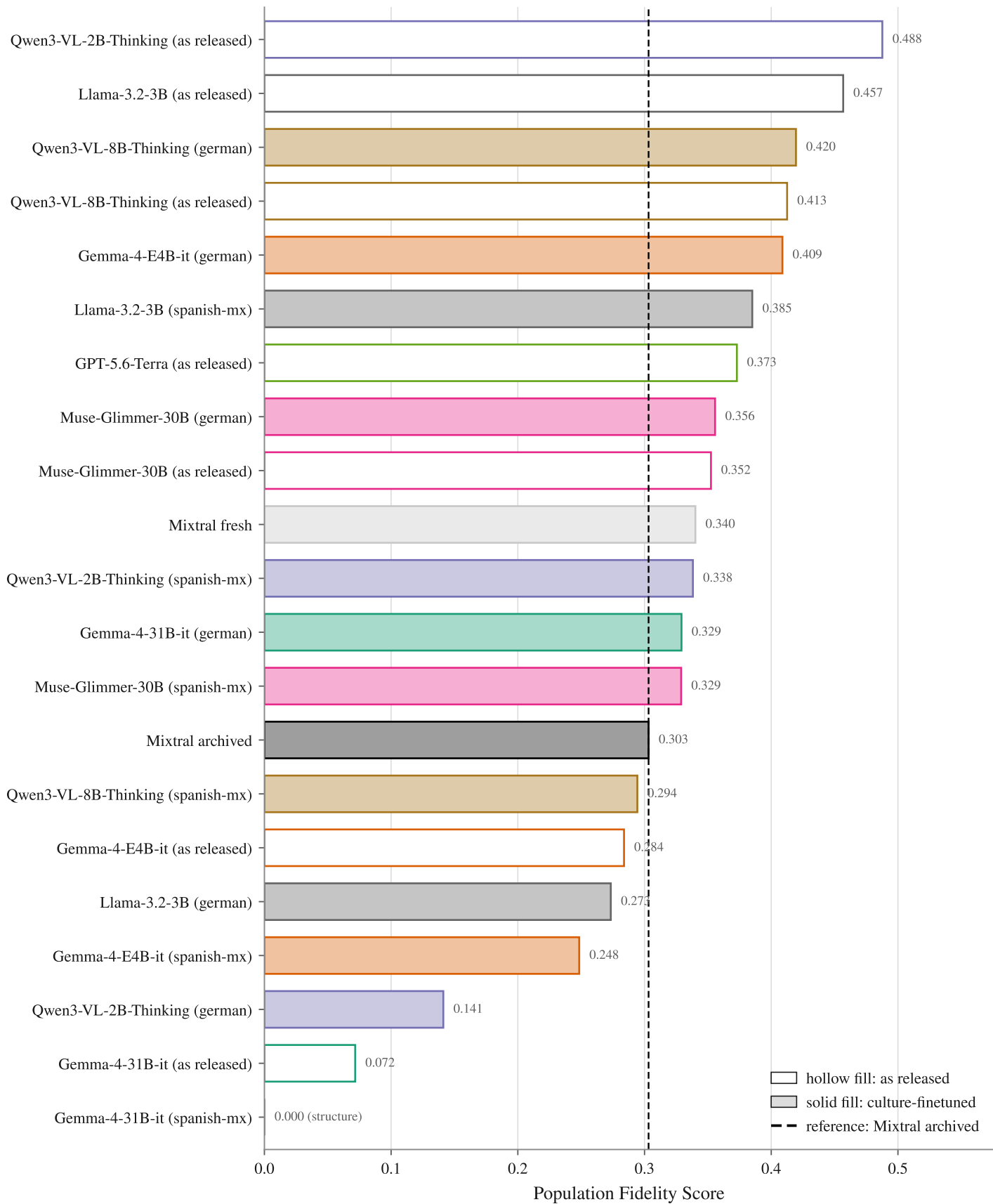
Population fidelity — happiness, FA
