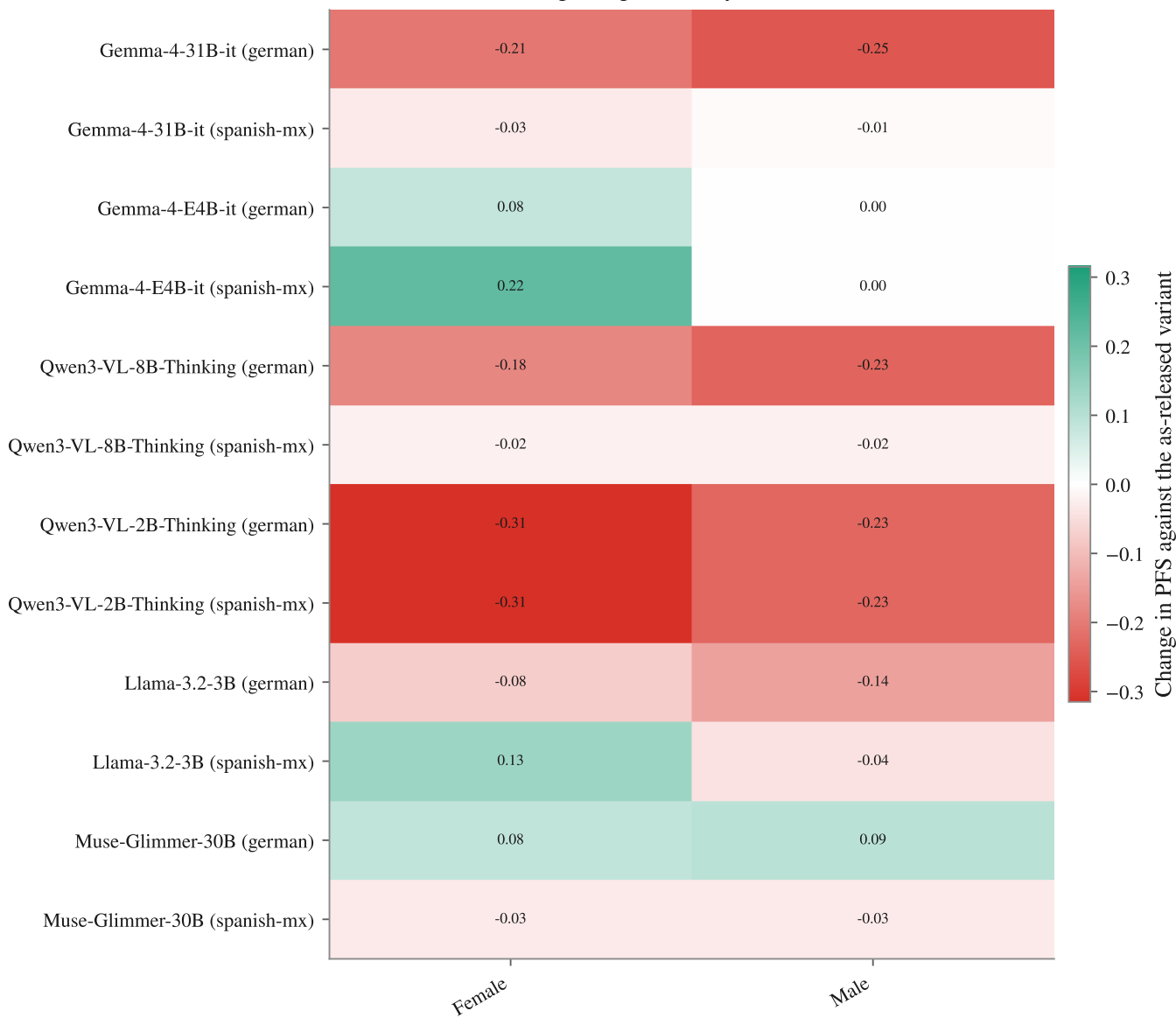
Finetuning change in fidelity — Sex, trust, NTP
