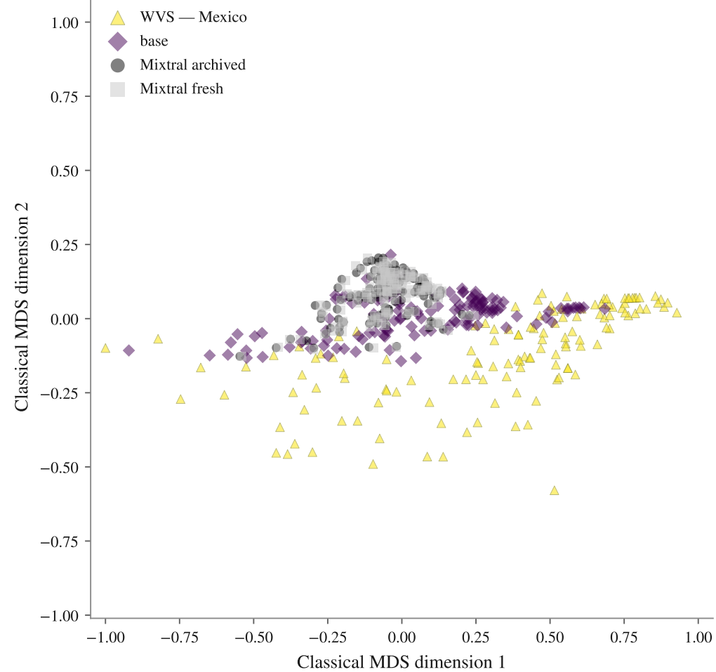
FA · 131 subpopulations · mean nEMD base 0.122, Mixtral archived 0.109, Mixtral fresh 0.125
