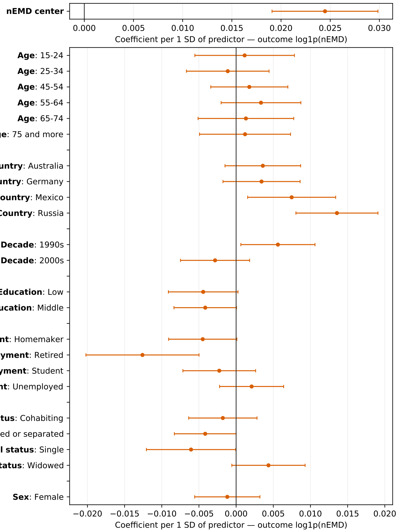
NTP (adj. R^2 = 0.302 )
