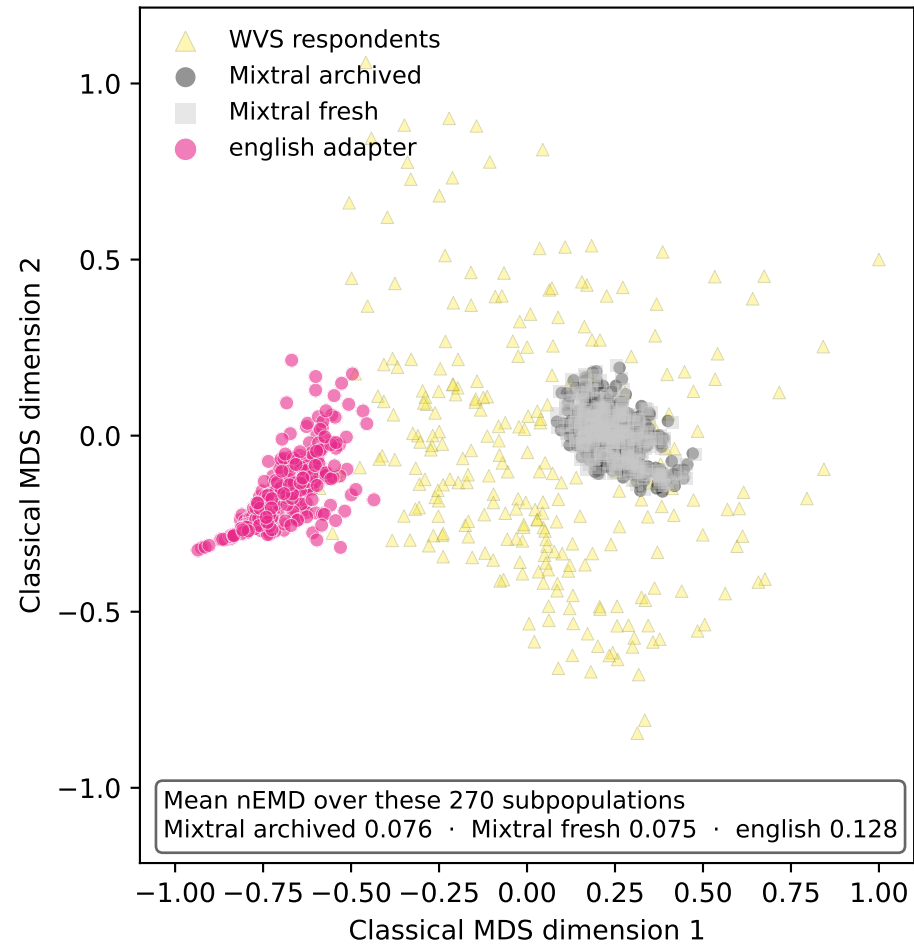
Next-token probabilities
