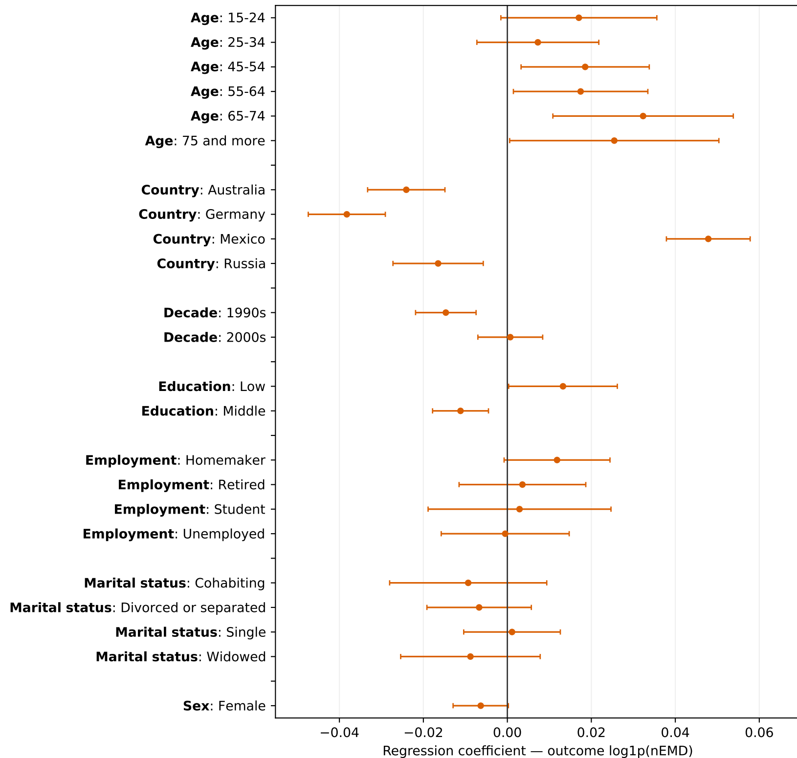
NTP (adj. R^2 = 0.461 )
