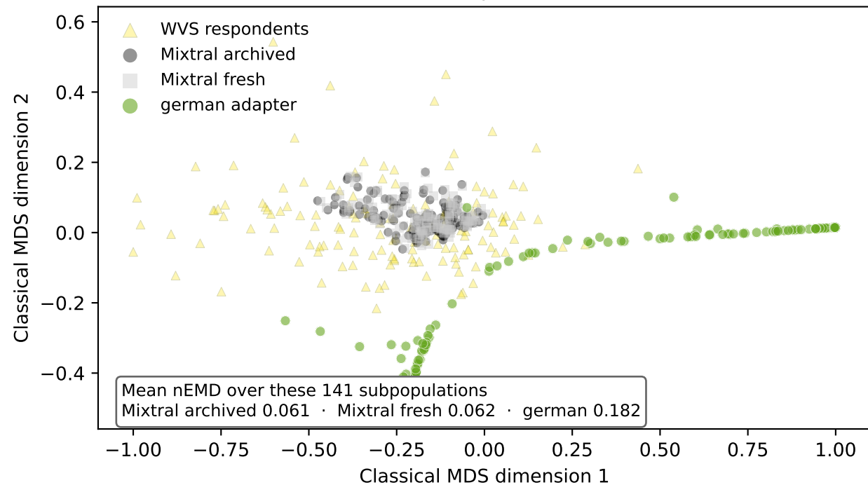
Next-token probabilities
