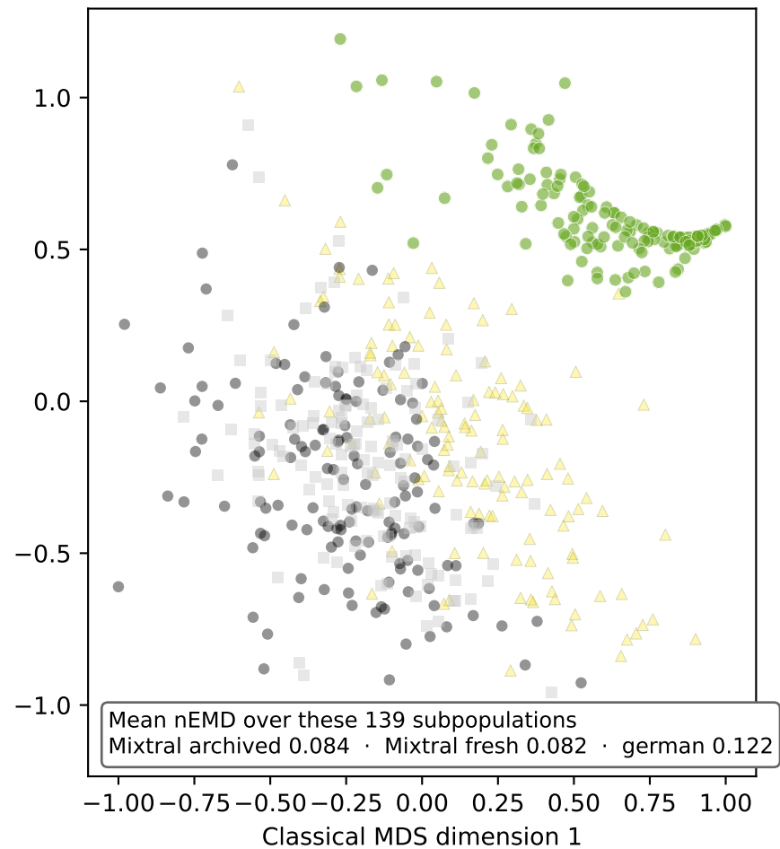
Full answer
