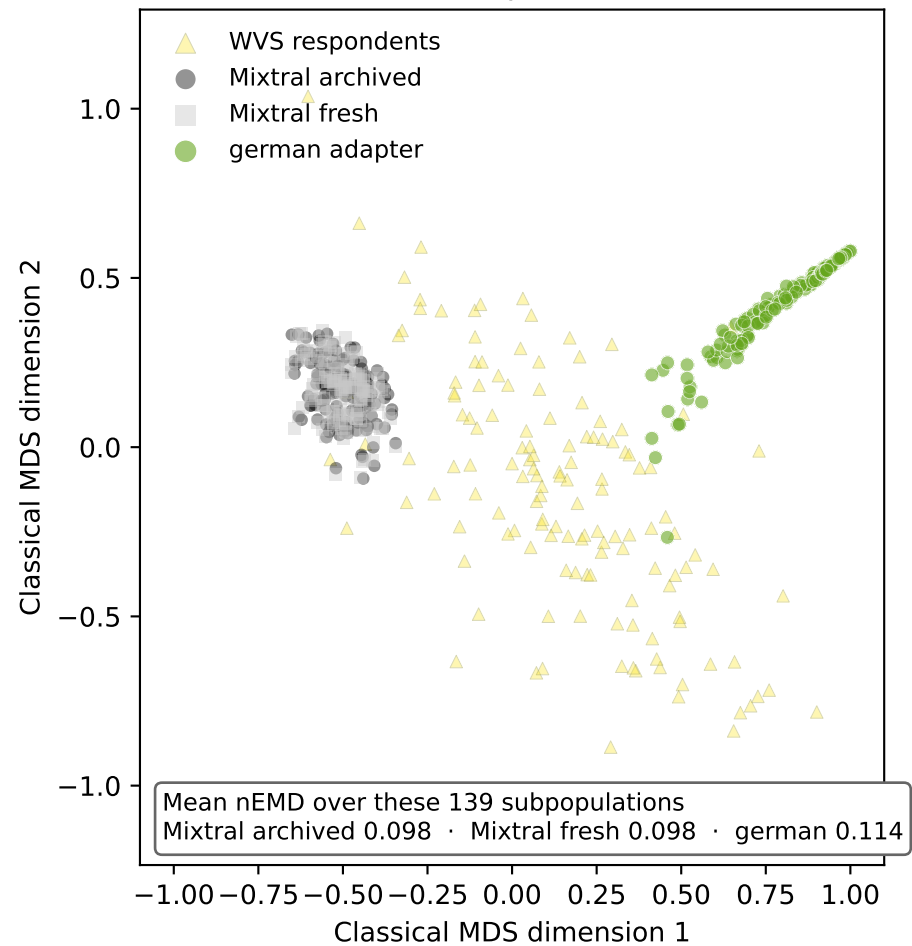
Next-token probabilities
