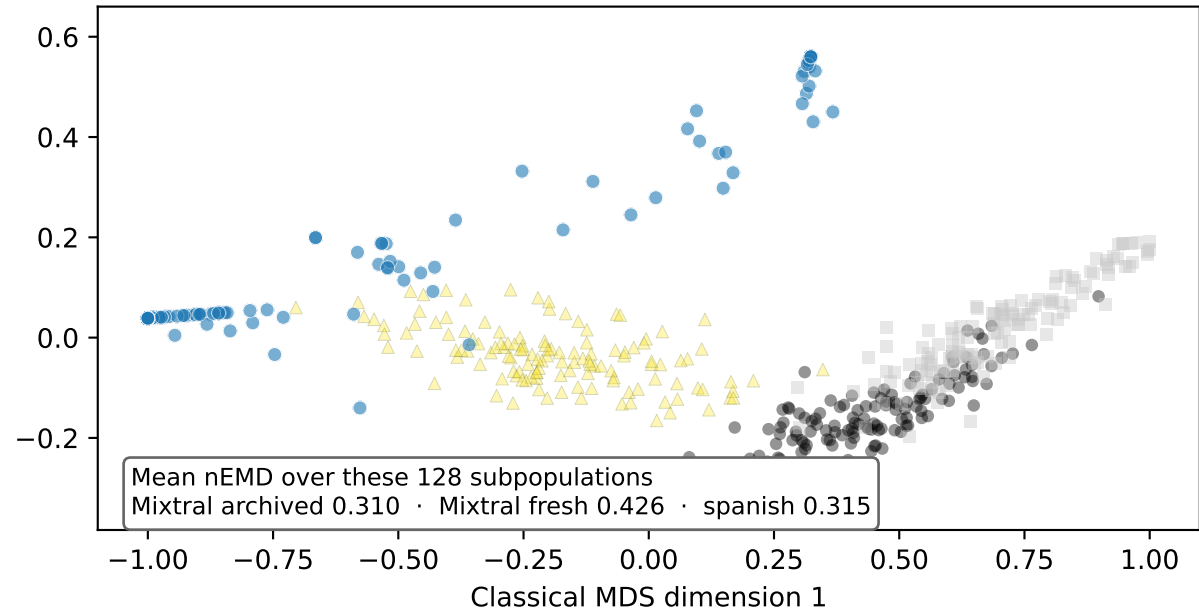
Full answer
