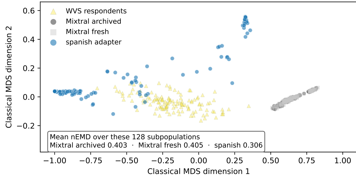
Next-token probabilities
