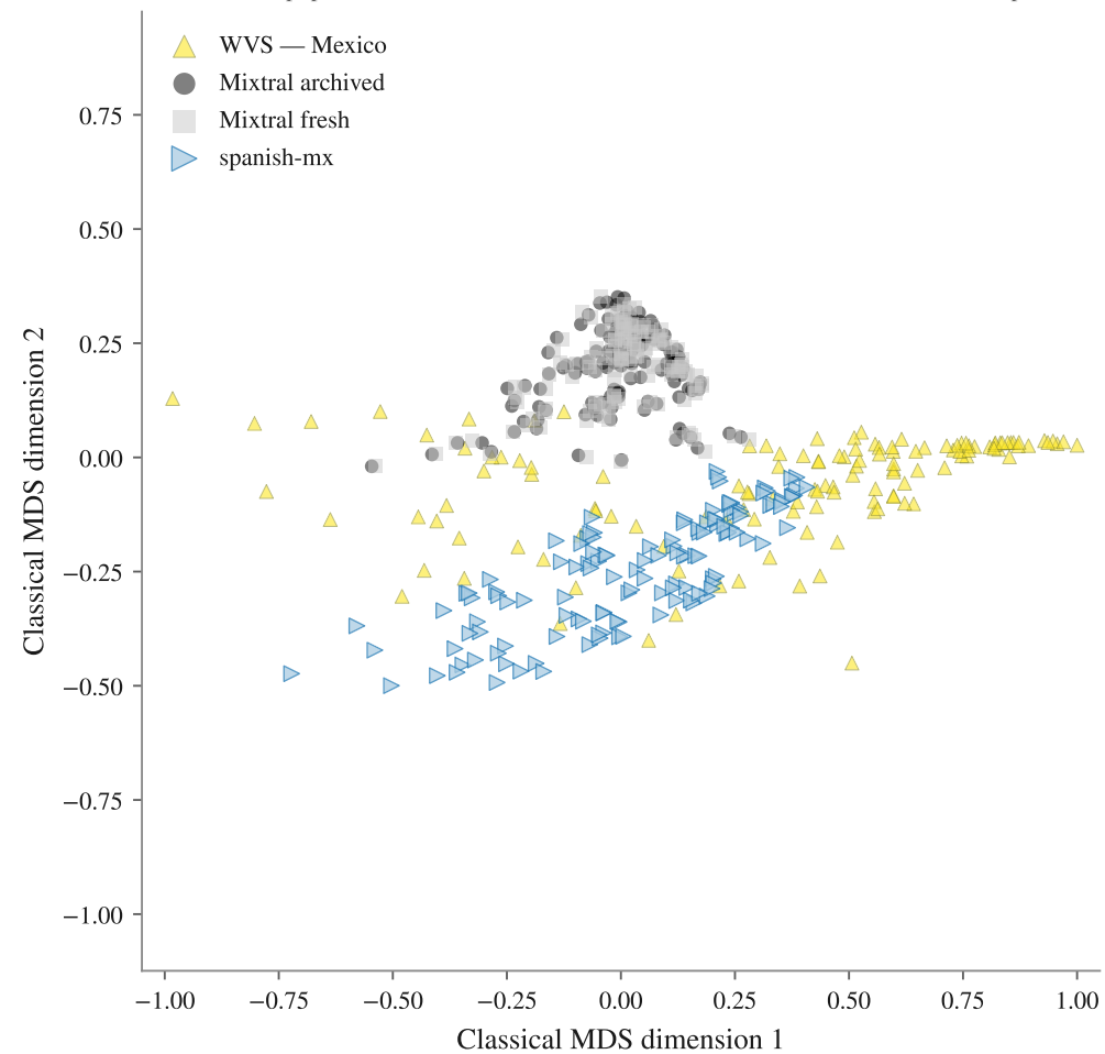
NTP · 131 subpopulations · mean nEMD Mixtral archived 0.122, Mixtral fresh 0.121, spanish-mx 0.120
