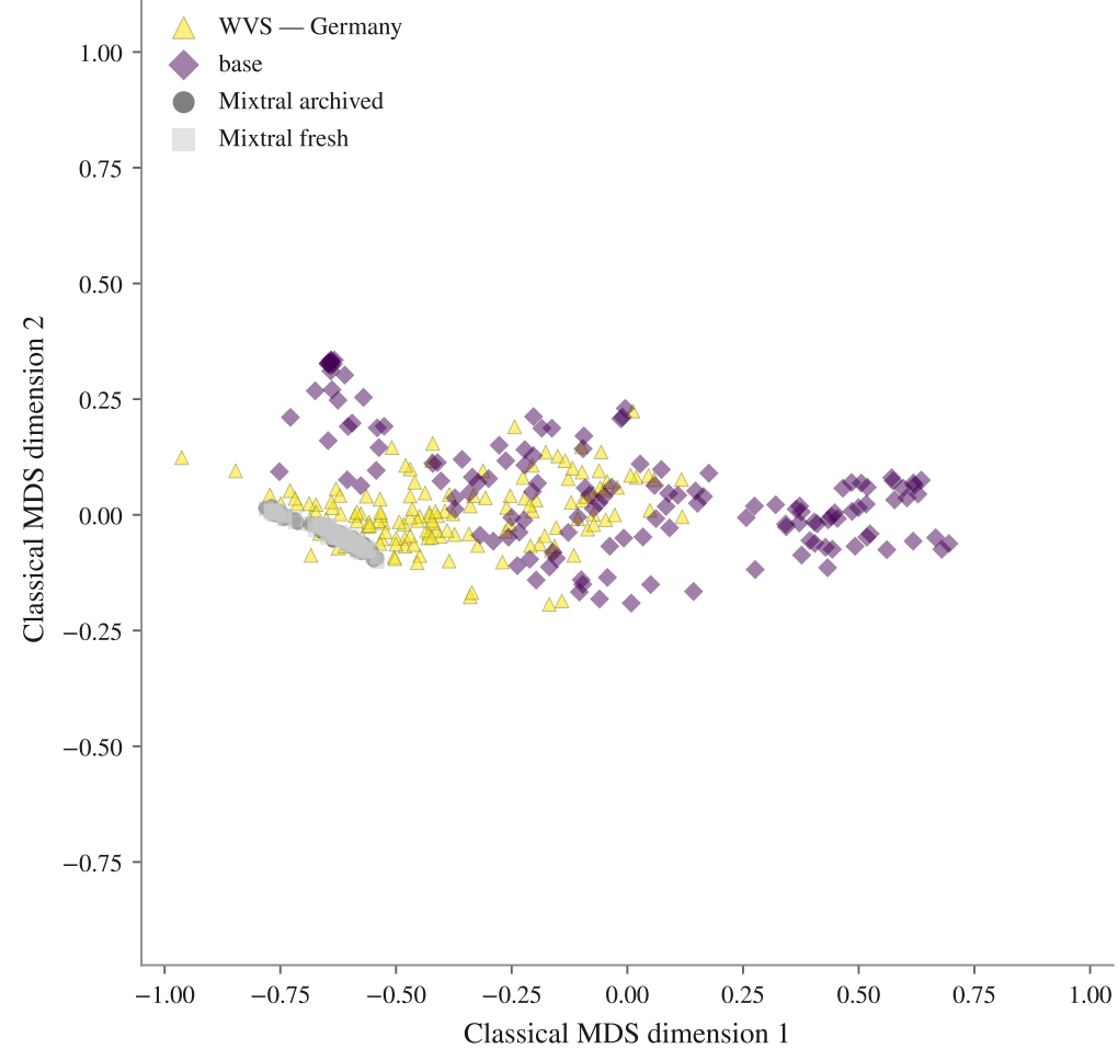
FA · 141 subpopulations · mean nEMD base 0.265, Mixtral archived 0.156, Mixtral fresh 0.175
