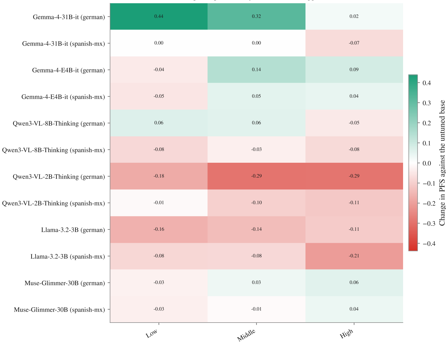
Finetuning change in fidelity — Education, happiness, NTP
