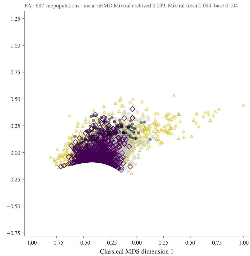
Muse-Glimmer-30B
