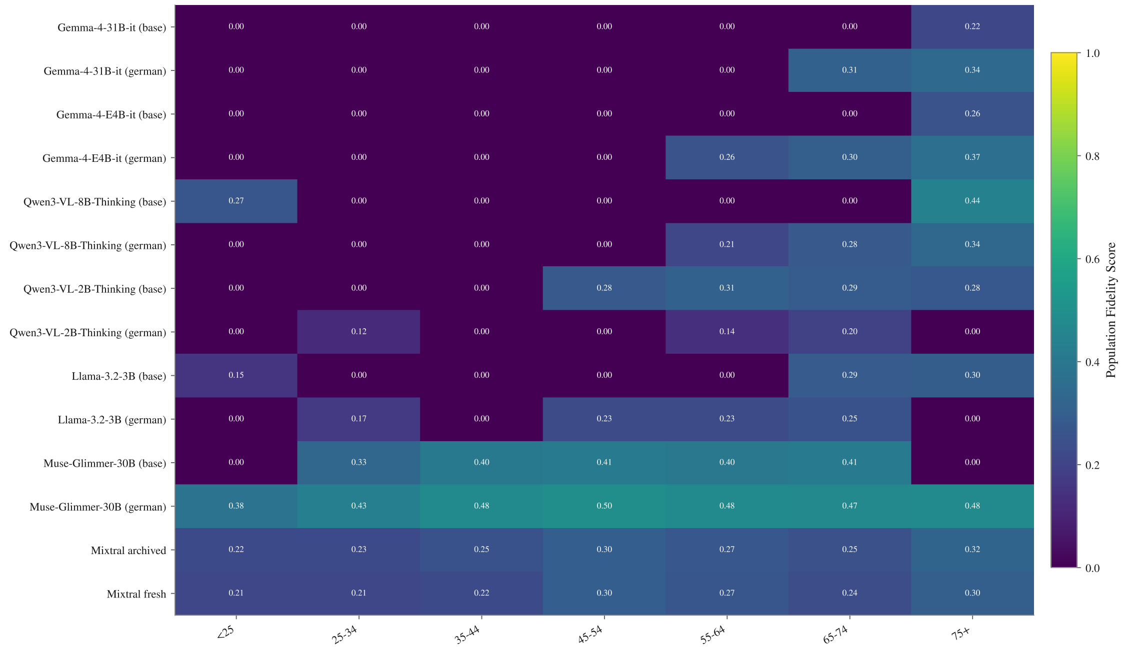
Population fidelity — Age band, every topic, NTP
