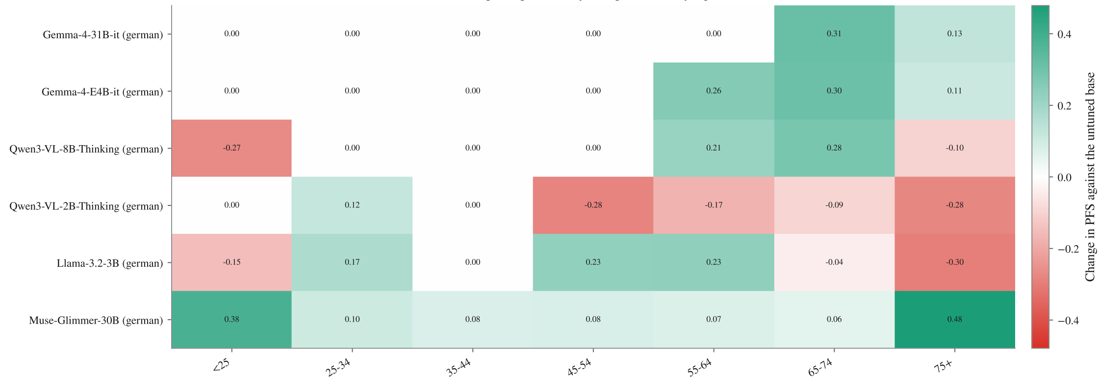
Finetuning change in fidelity — Age band, every topic, NTP
