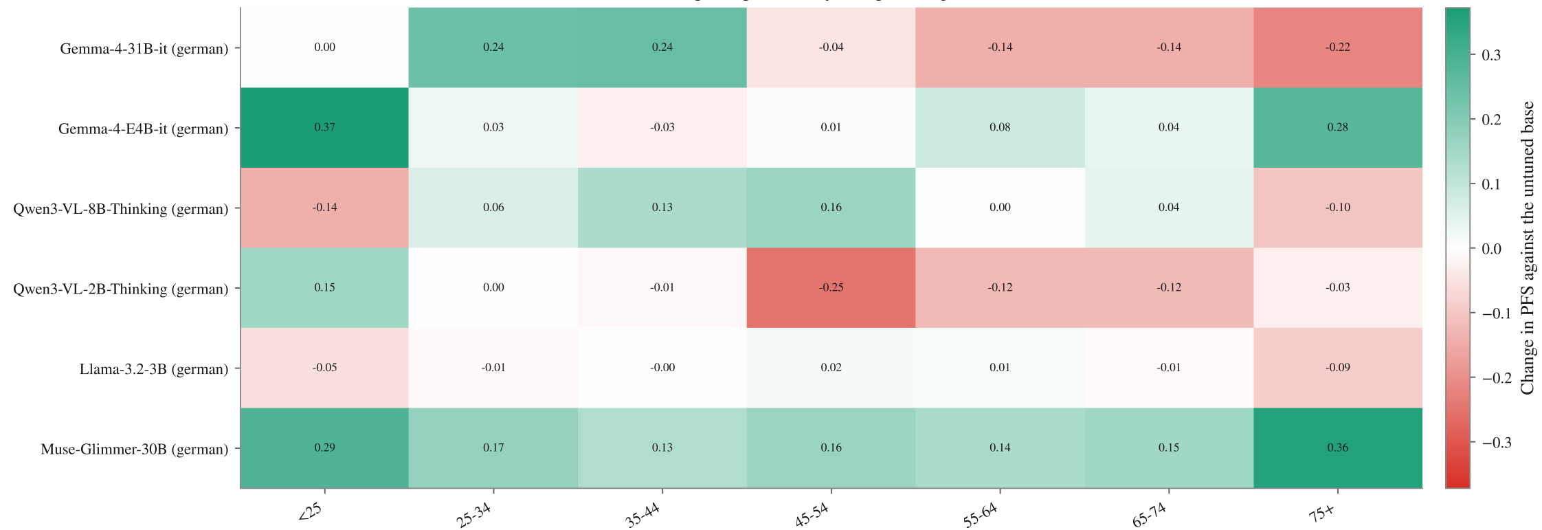
Finetuning change in fidelity — Age band, politics, NTP
