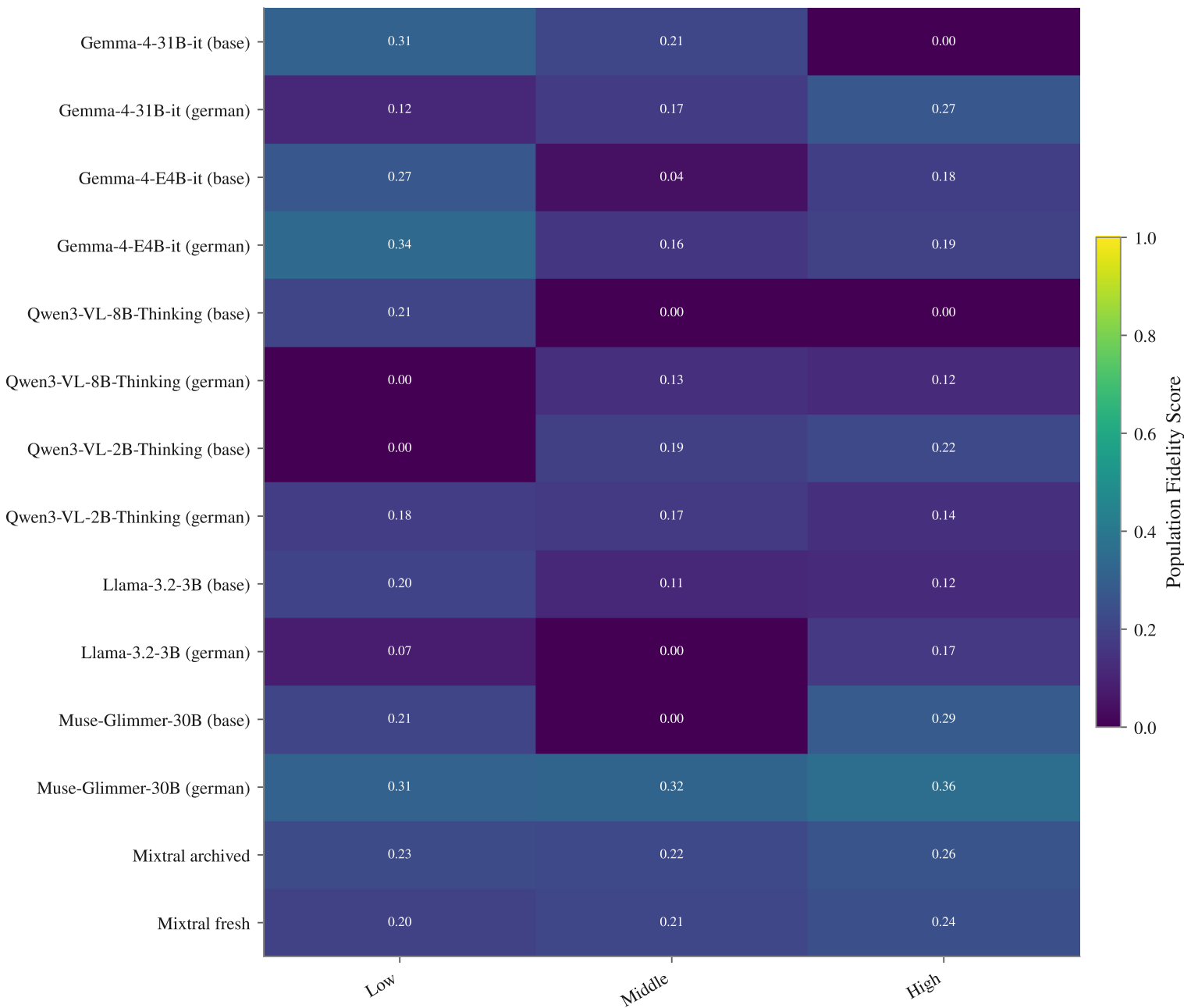
Population fidelity — Education, politics, NTP
