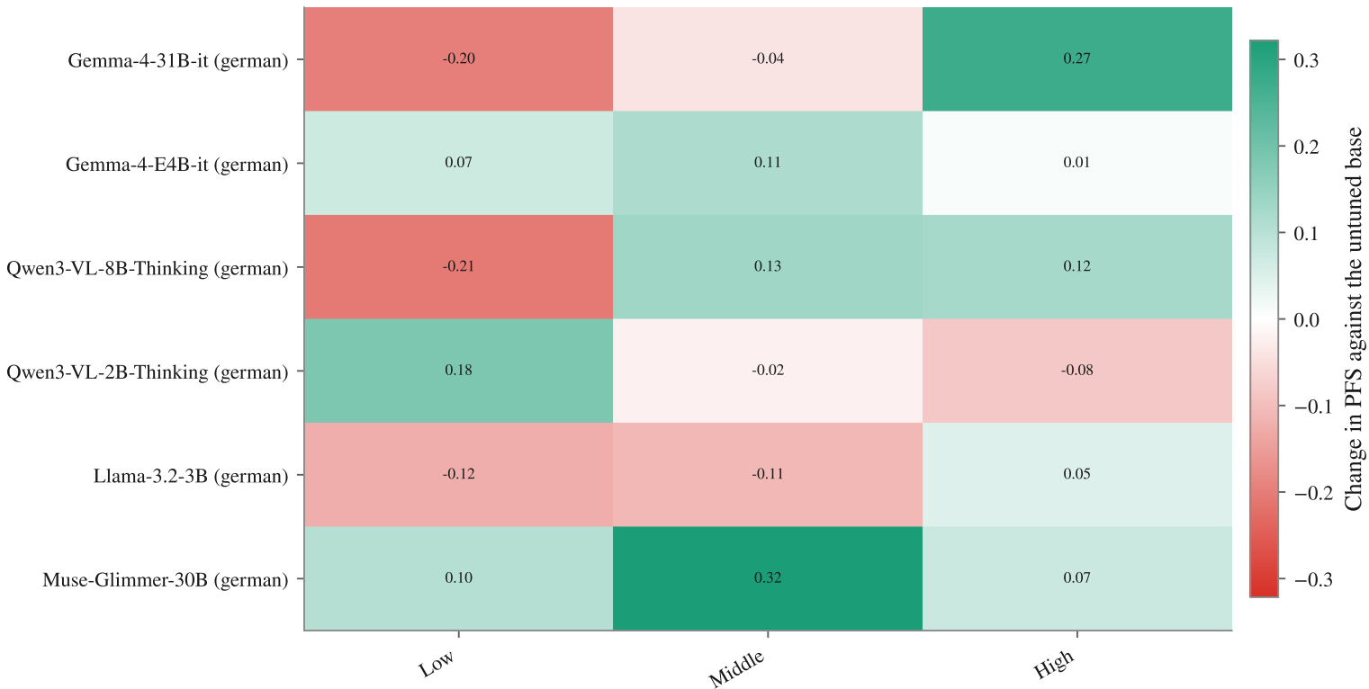
Finetuning change in fidelity — Education, politics, NTP
