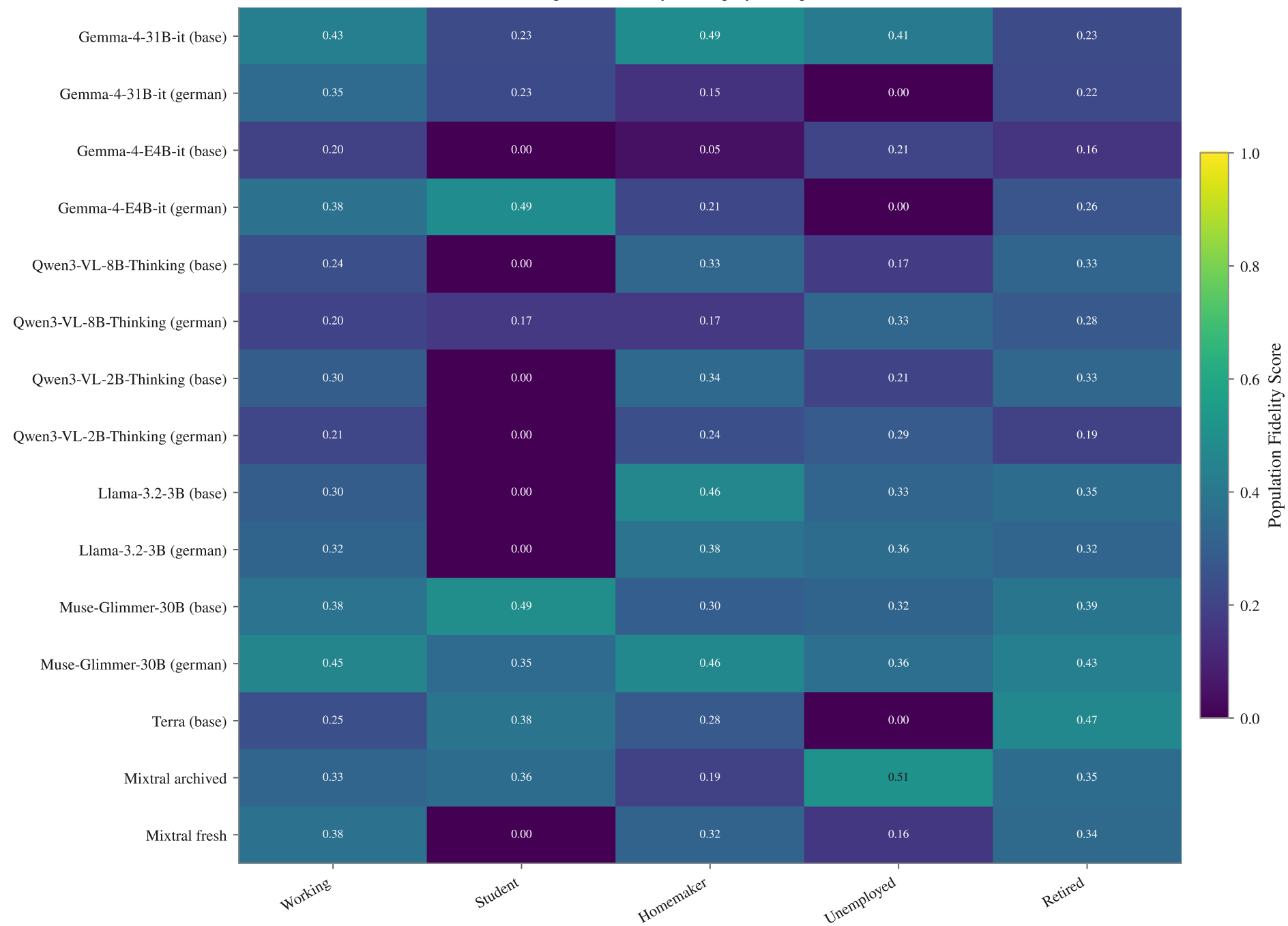
Population fidelity — Employment, politics, FA
