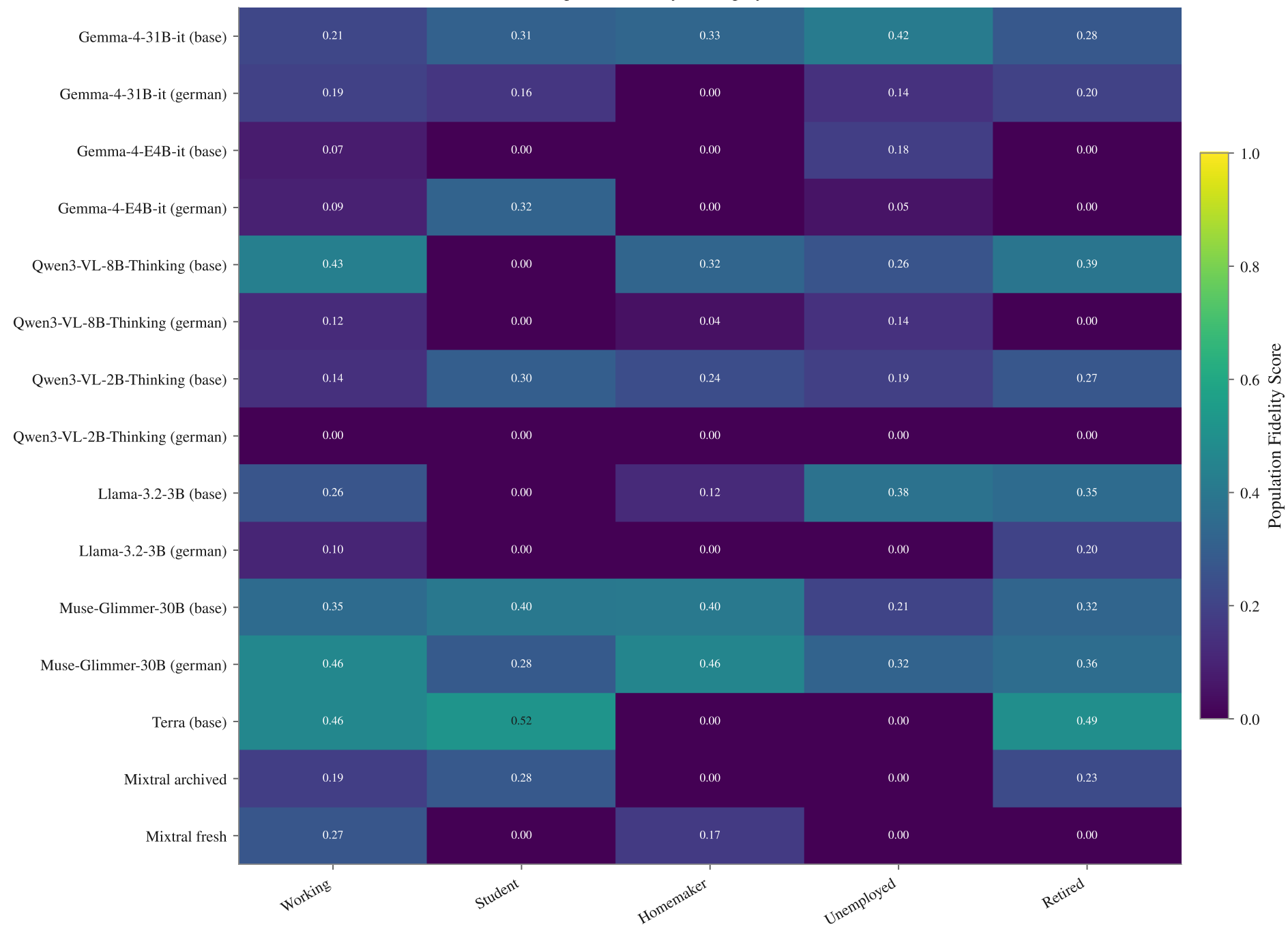
Population fidelity — Employment, trust, FA
