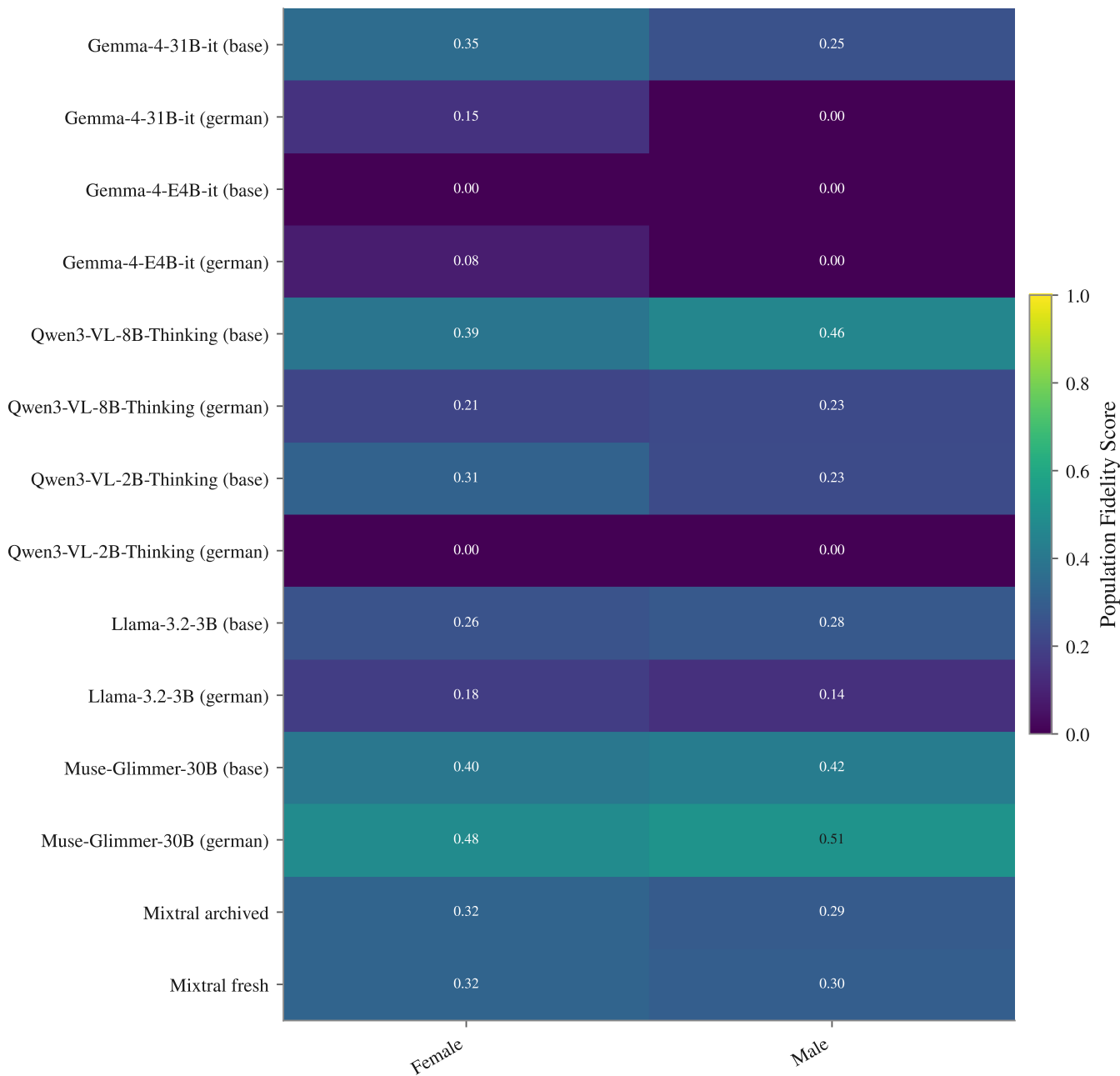
Population fidelity — Sex, trust, NTP
