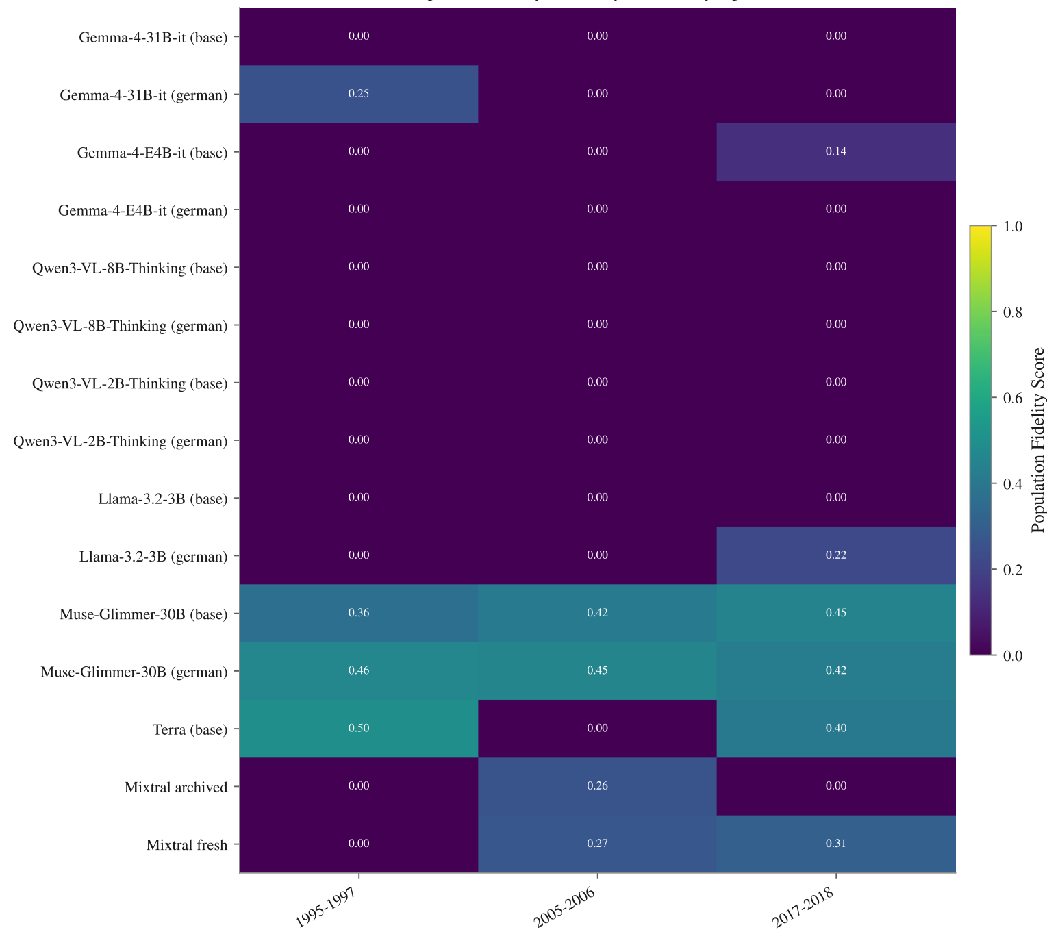
Population fidelity — Survey wave, every topic, FA
