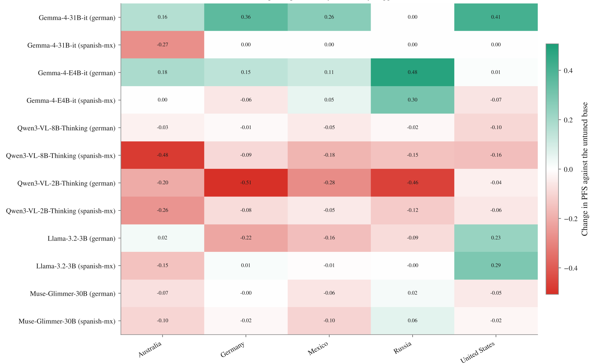
Finetuning change in fidelity — Country, happiness, FA
