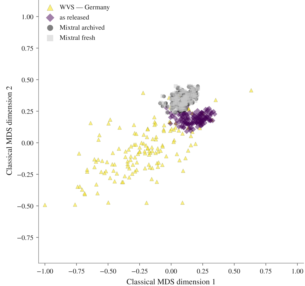
FA · 144 subpopulations · mean nEMD base 0.117, Mixtral archived 0.085, Mixtral fresh 0.083
