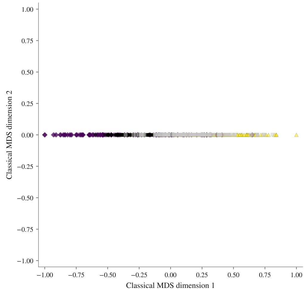
FA · 144 subpopulations · mean nEMD base 0.349, Mixtral archived 0.273, Mixtral fresh 0.146
