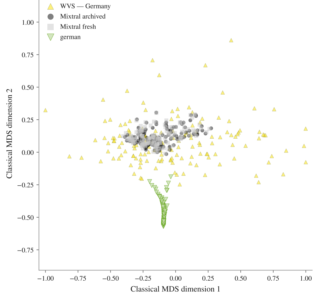
NTP · 144 subpopulations · mean nEMD Mixtral archived 0.062, Mixtral fresh 0.063, german 0.119
