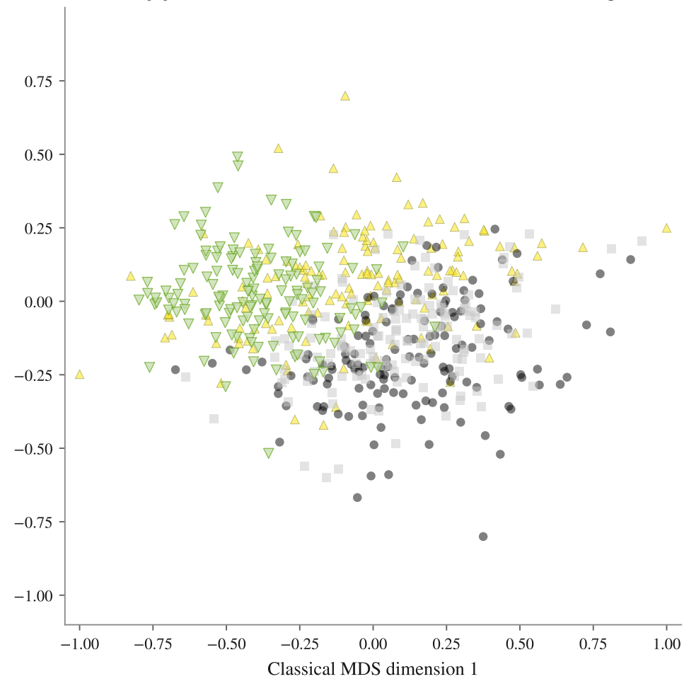
FA · 144 subpopulations · mean nEMD Mixtral archived 0.085, Mixtral fresh 0.083, german 0.088
