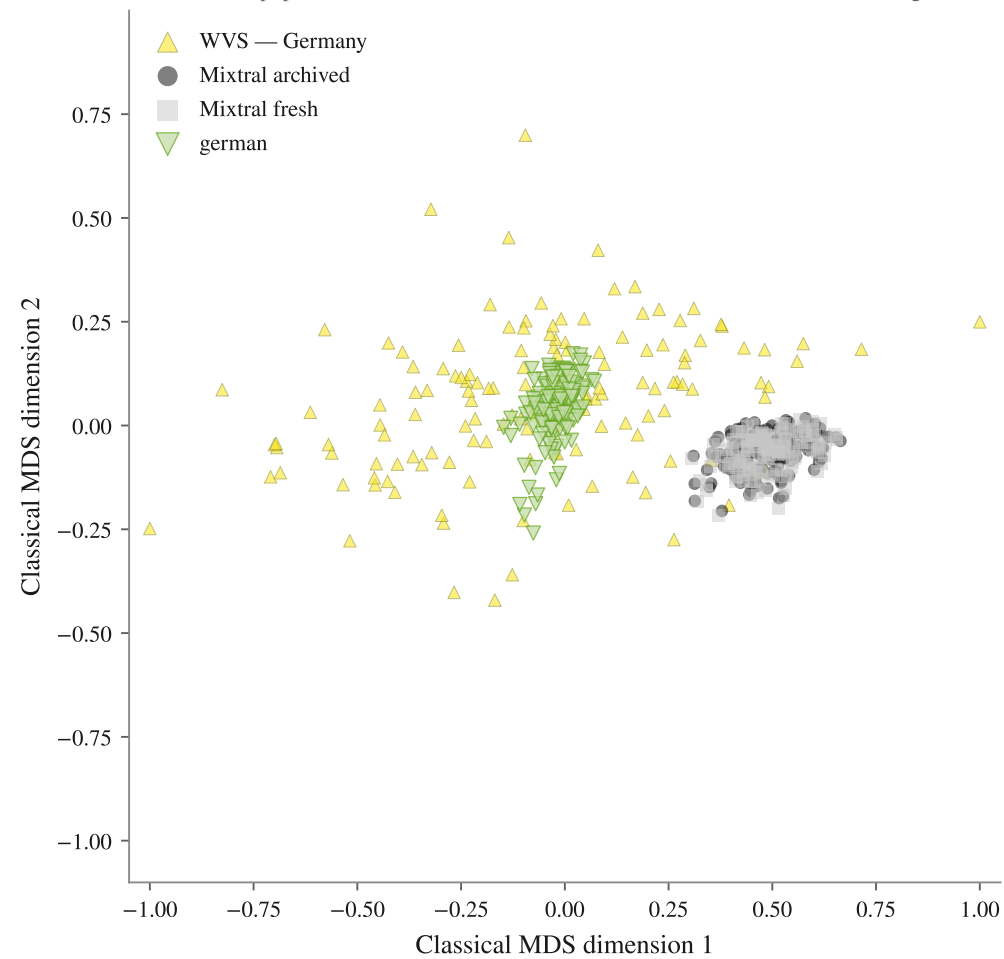
NTP · 144 subpopulations · mean nEMD Mixtral archived 0.099, Mixtral fresh 0.099, german 0.058
