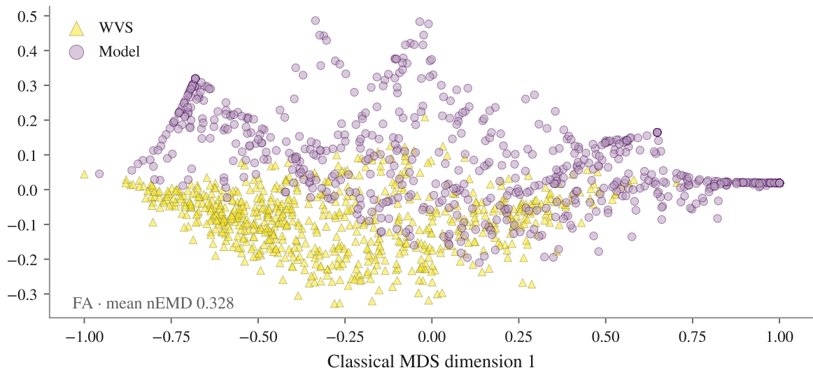
Classical MDS dimension 2
