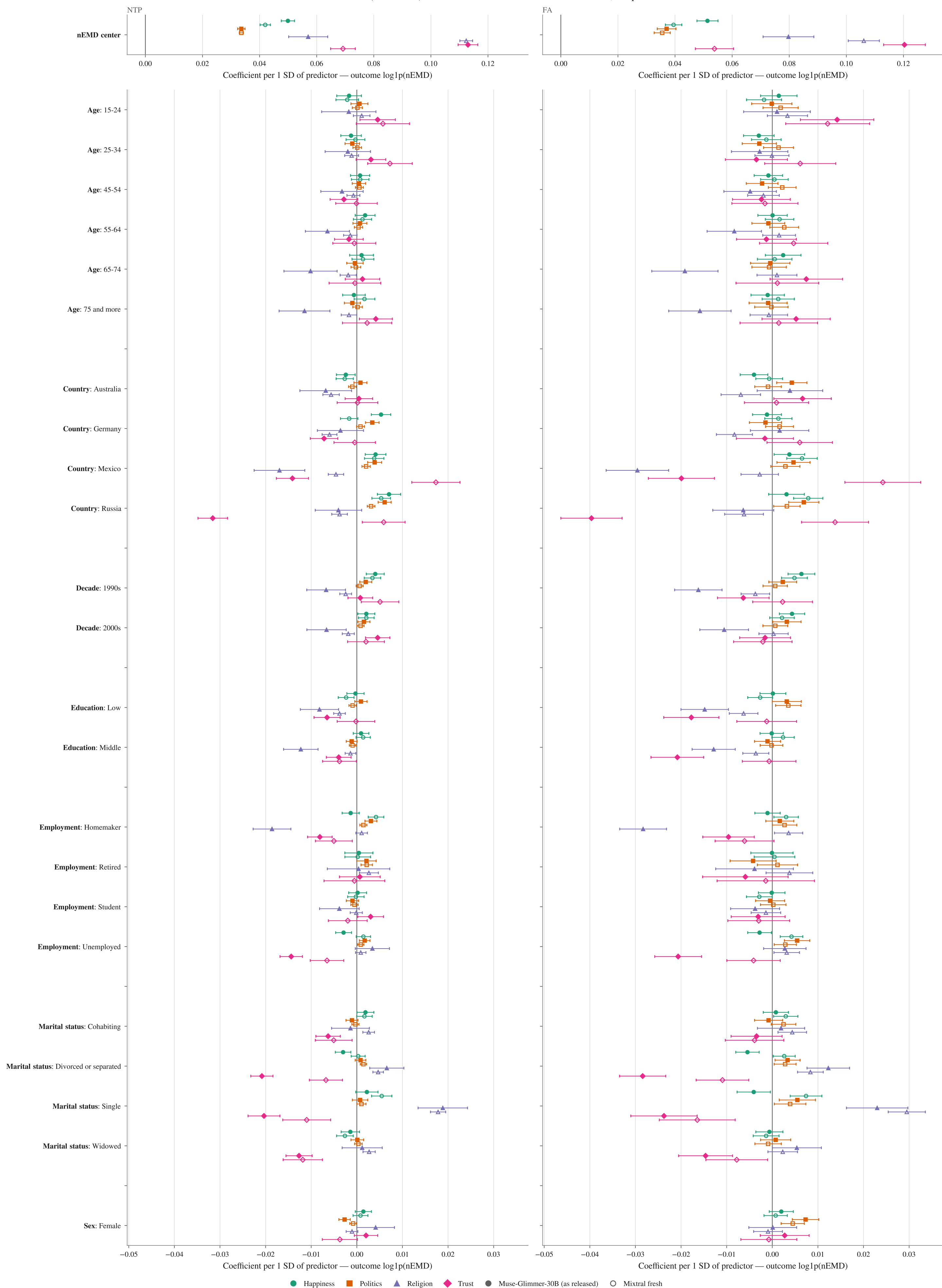
Muse-Glimmer-30B (as released) vs Mixtral fresh — standardized coefficients, all questions
