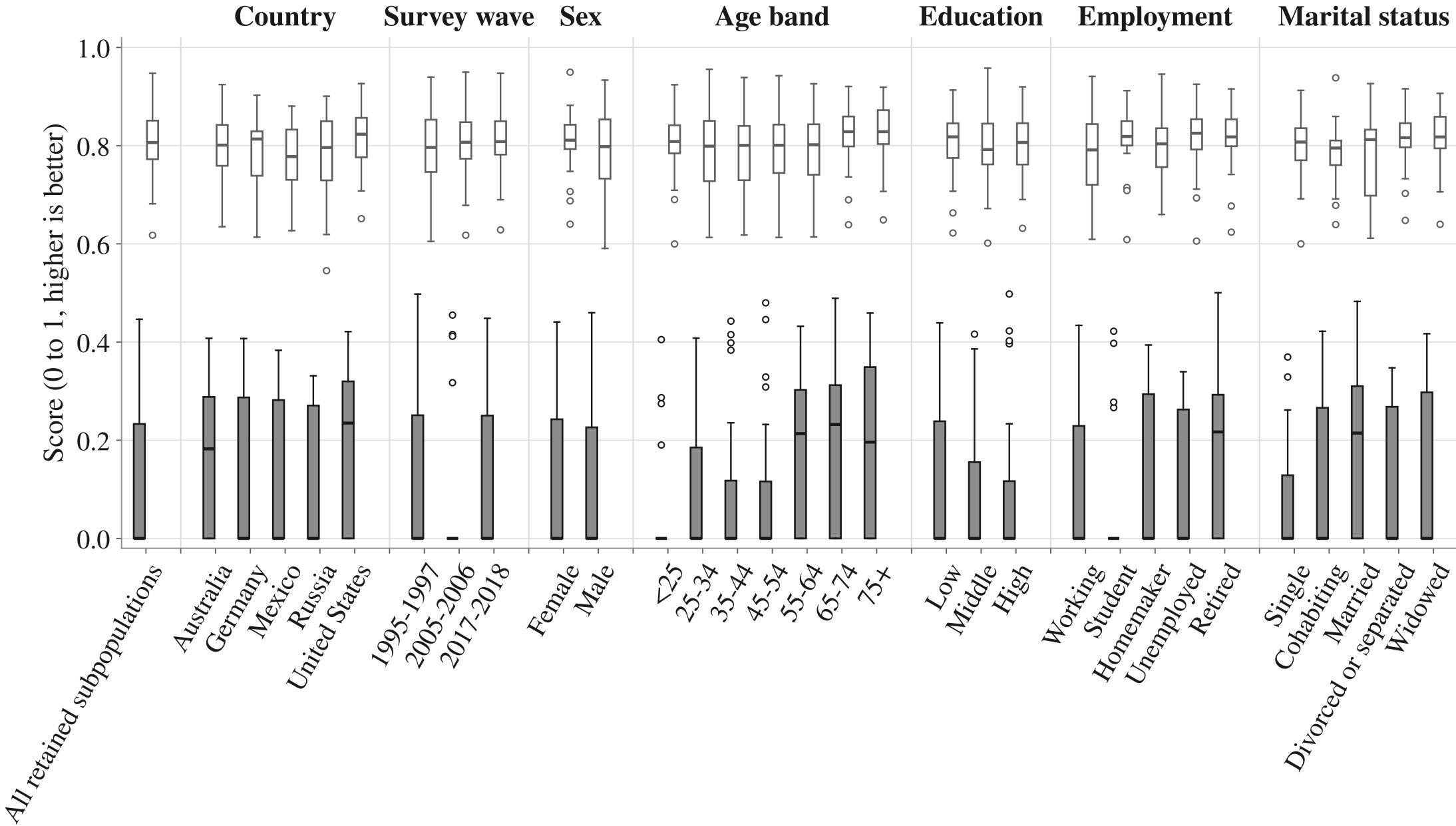
Population Fidelity Score Center: 1 - C (not in PFS) boxes span the model conditions (FA 19); Mixtral references excluded
