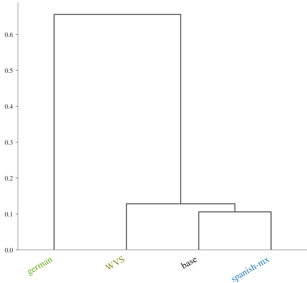
mean nEMD between variants
