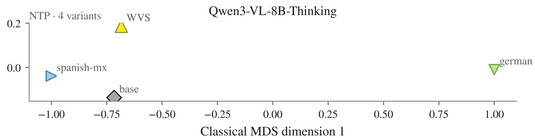
Classical MDS dimension 2
