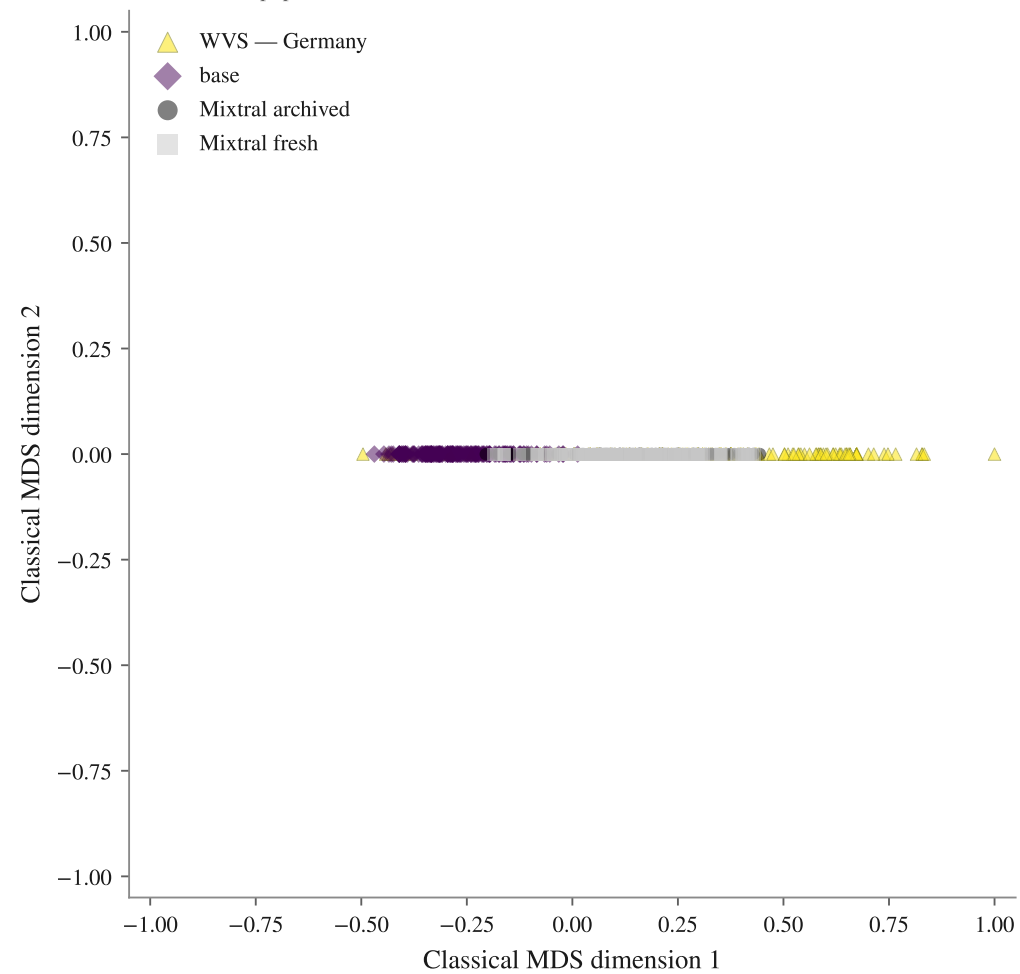
FA · 144 subpopulations · mean nEMD base 0.301, Mixtral archived 0.273, Mixtral fresh 0.146
