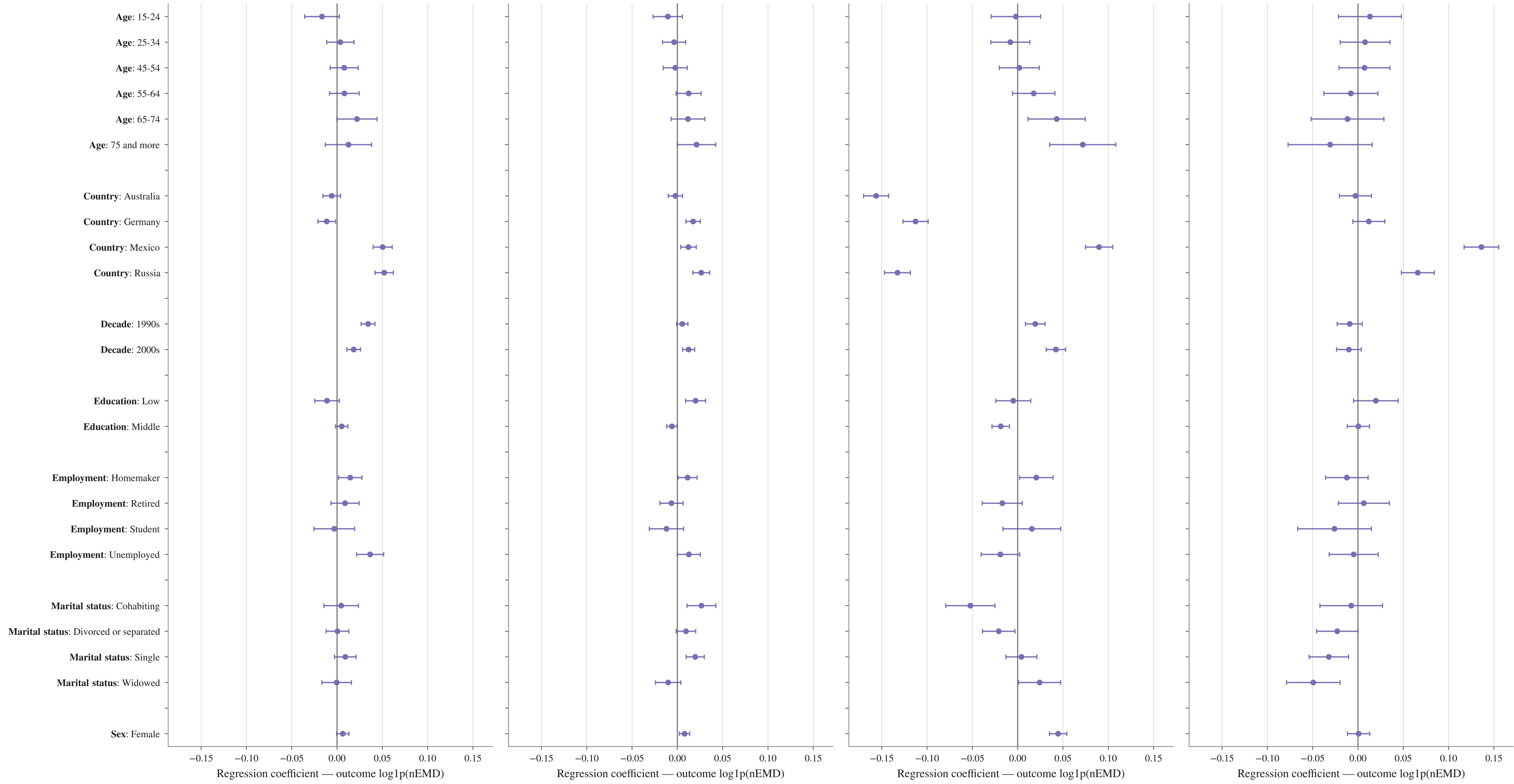
Happiness · adj. R^2 = 0.383
