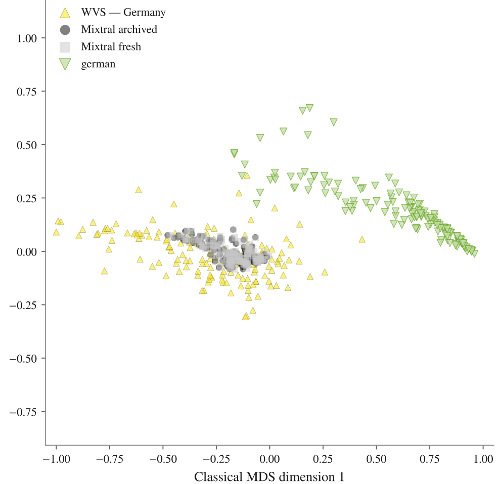
FA · 144 subpopulations · mean nEMD Mixtral archived 0.092, Mixtral fresh 0.074, german 0.268
