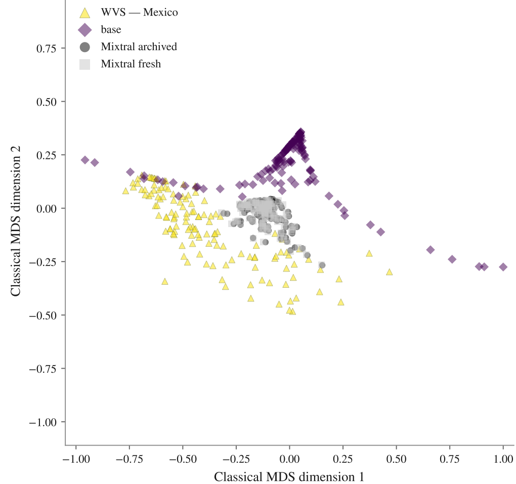
FA · 131 subpopulations · mean nEMD base 0.197, Mixtral archived 0.109, Mixtral fresh 0.125
